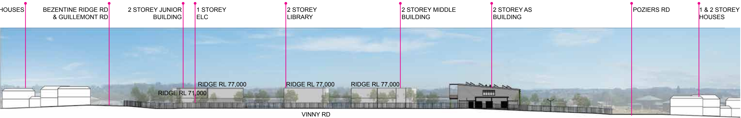
EAST ELEVATION
