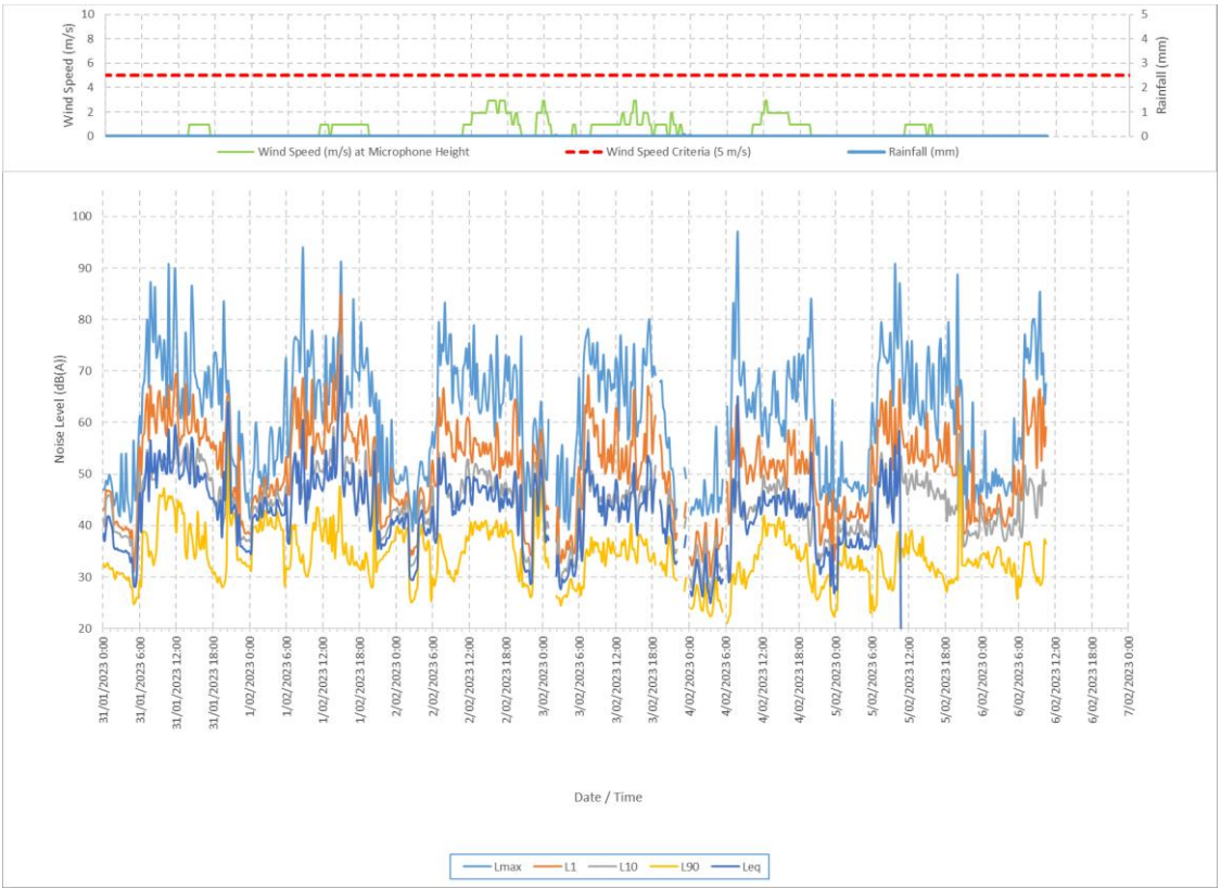
Figure 14: Time History from 31/01/2023 to 6/02/2023 at ML2
