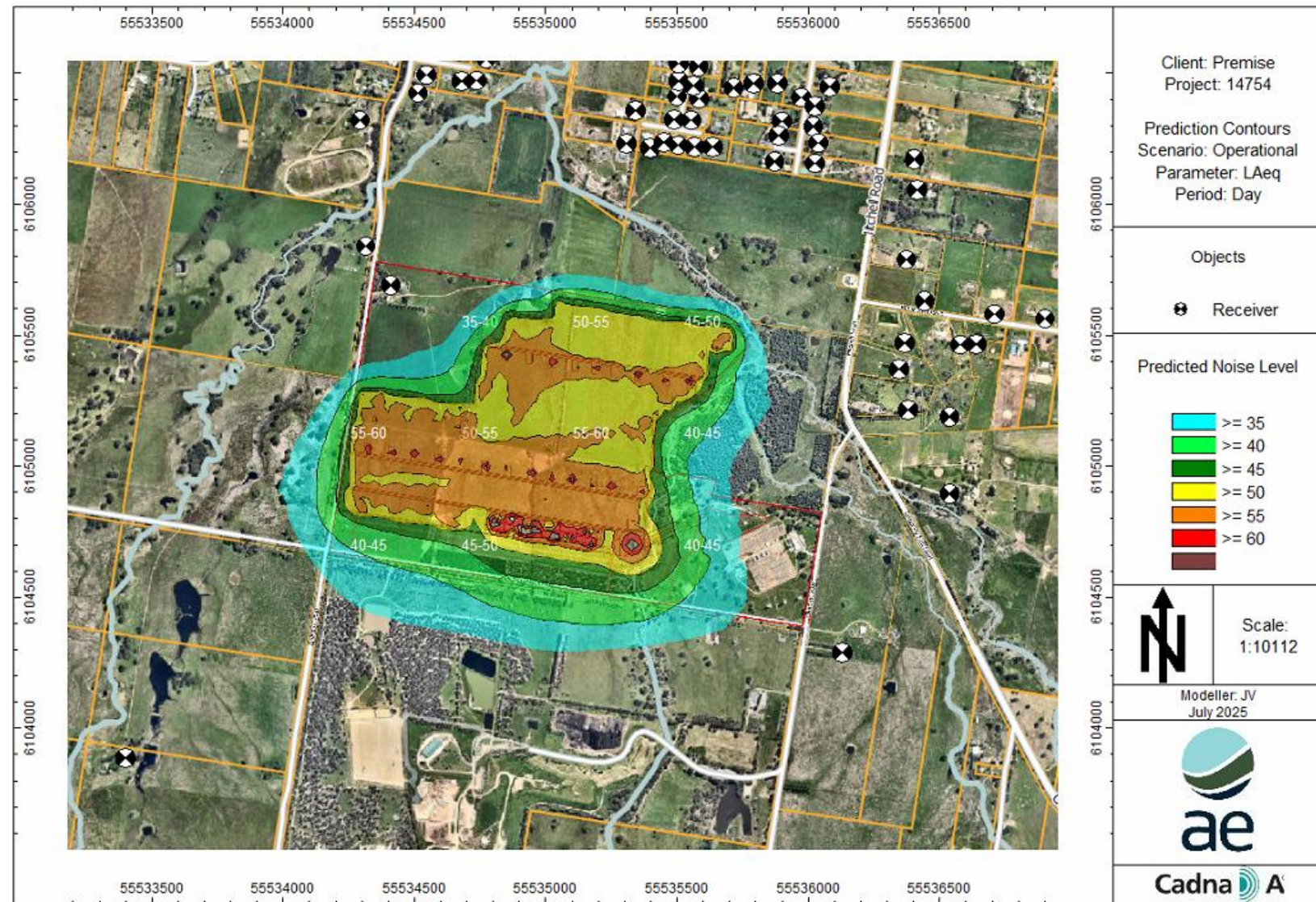
Figure 15: Predicted Operational Noise Contours - Day
