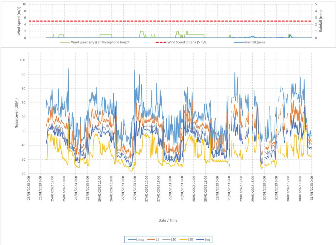
Figure 13: Time History from 25/01/2023 to 31/01/2023 at ML2
