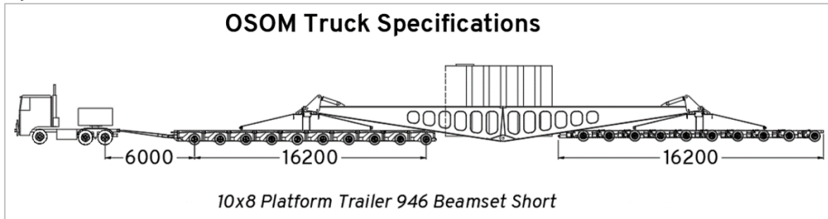
Figure 9: OSOM Vehicle
