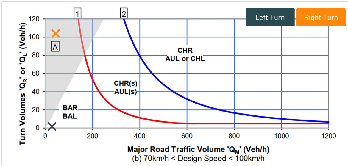
Figure 12: Figure 3.25 of Austrroads Guide to Traffic Management Part 6
