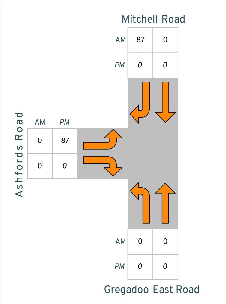
Figure 7: Construction Peak Hour Volumes During Peak Construction
