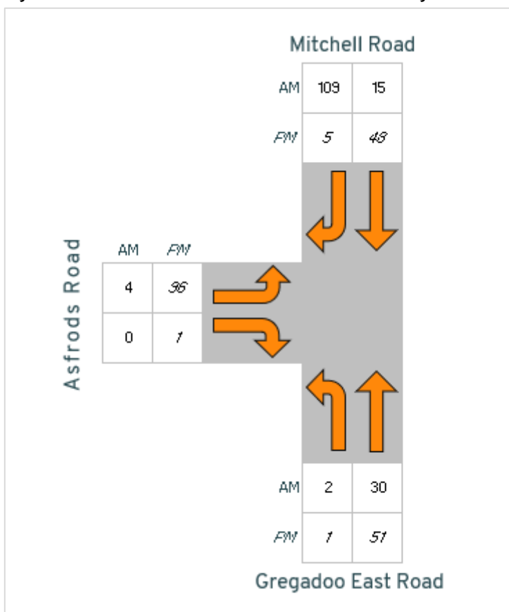
Figure 8: Total Construction Peak Hour Volumes During Peak Construction
