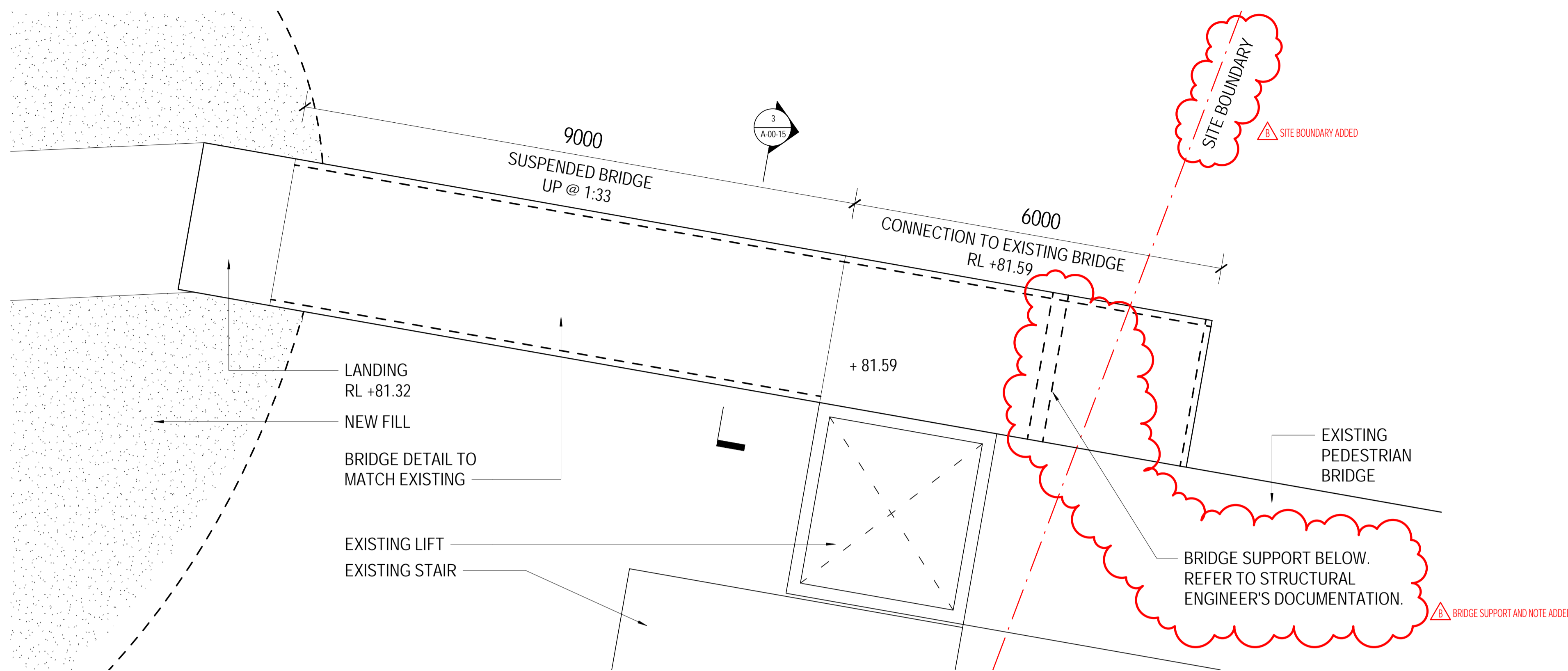
1 PLAN - BRIDGE
