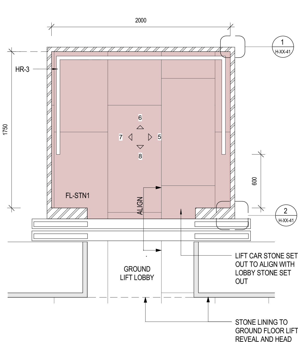
1 TYPICAL LIFT CAR DETAIL PLAN
