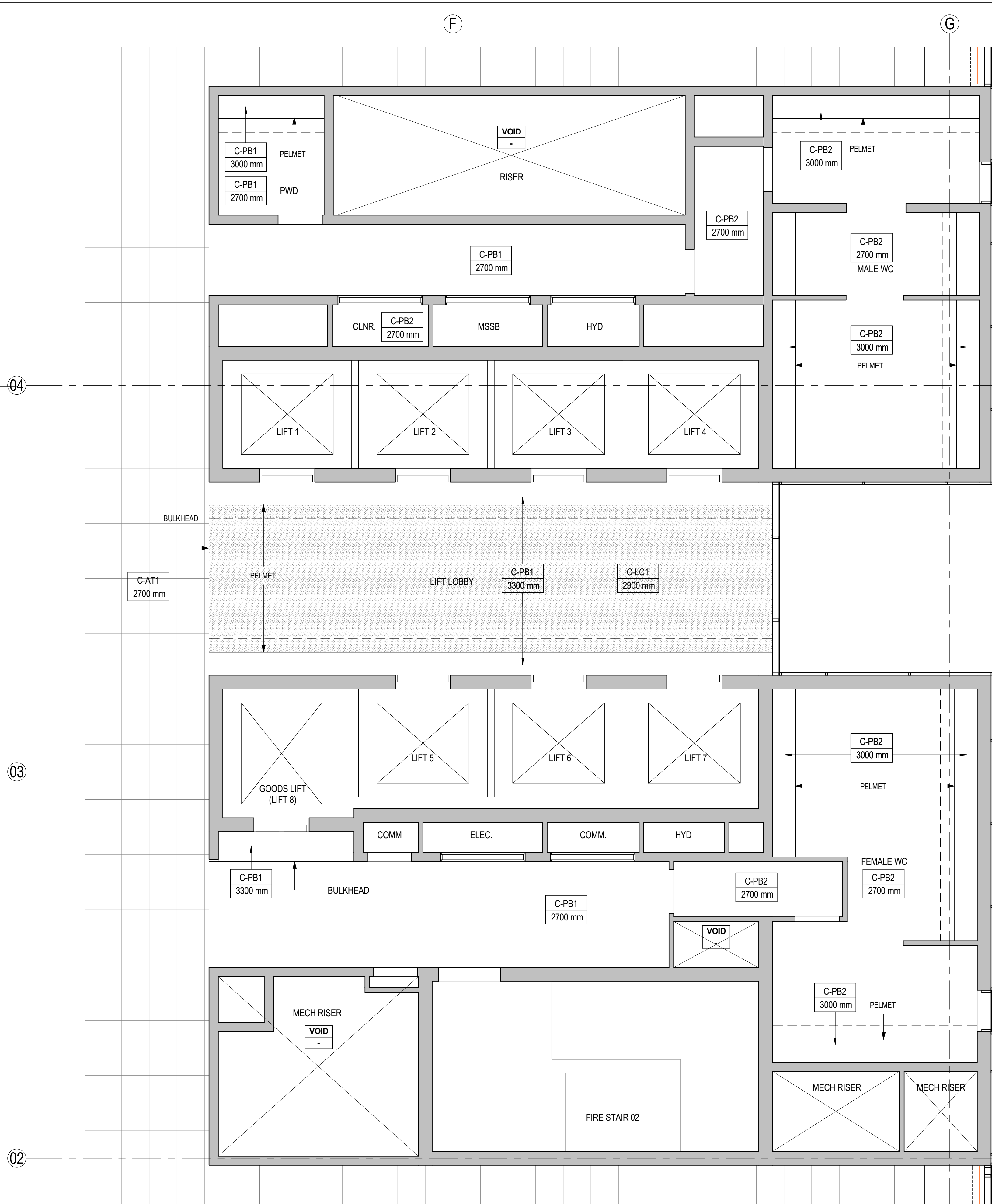
2 RCP - WARM SHELL CORE
