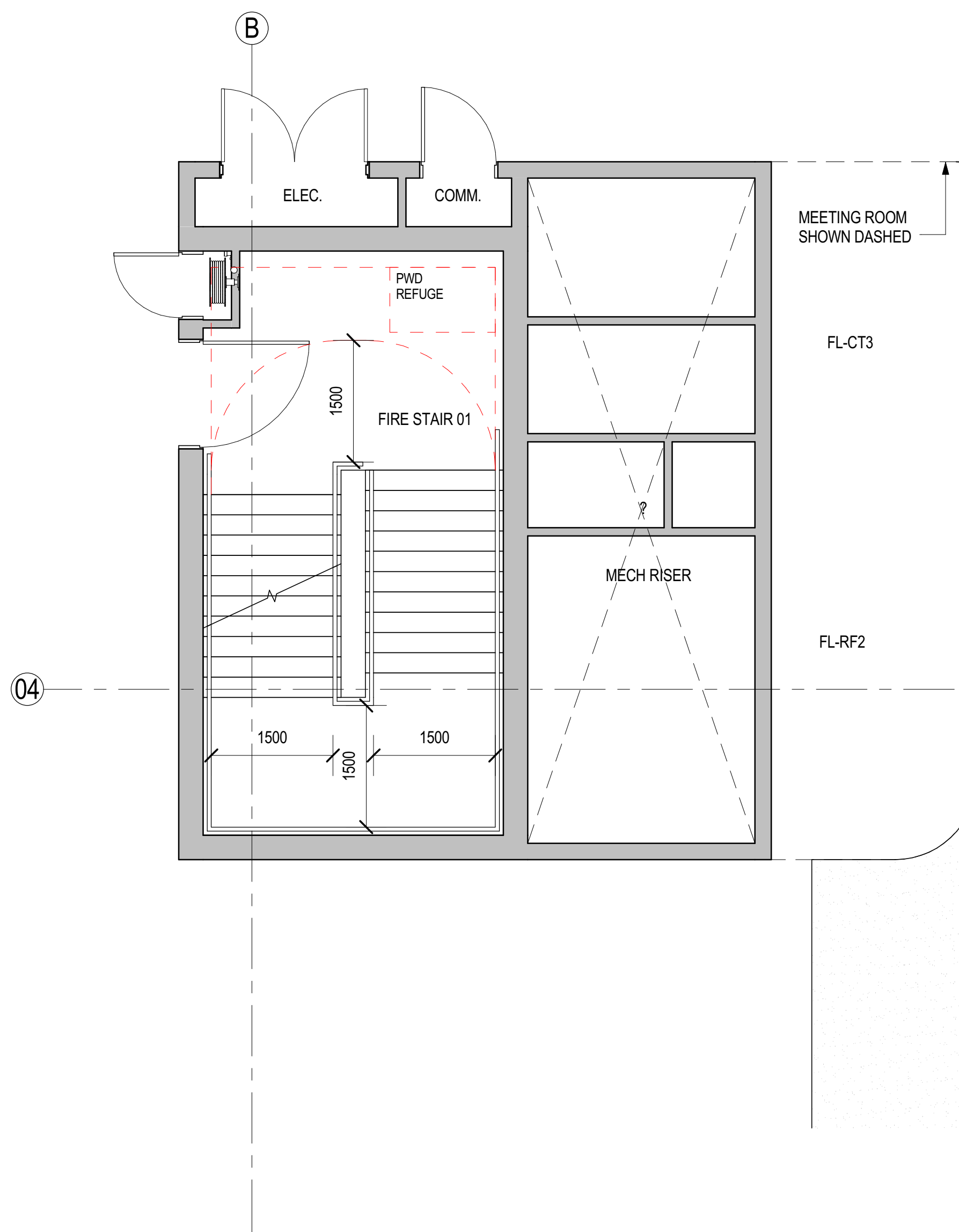
1 TYPICAL CORE - LEVEL 02 WEST
