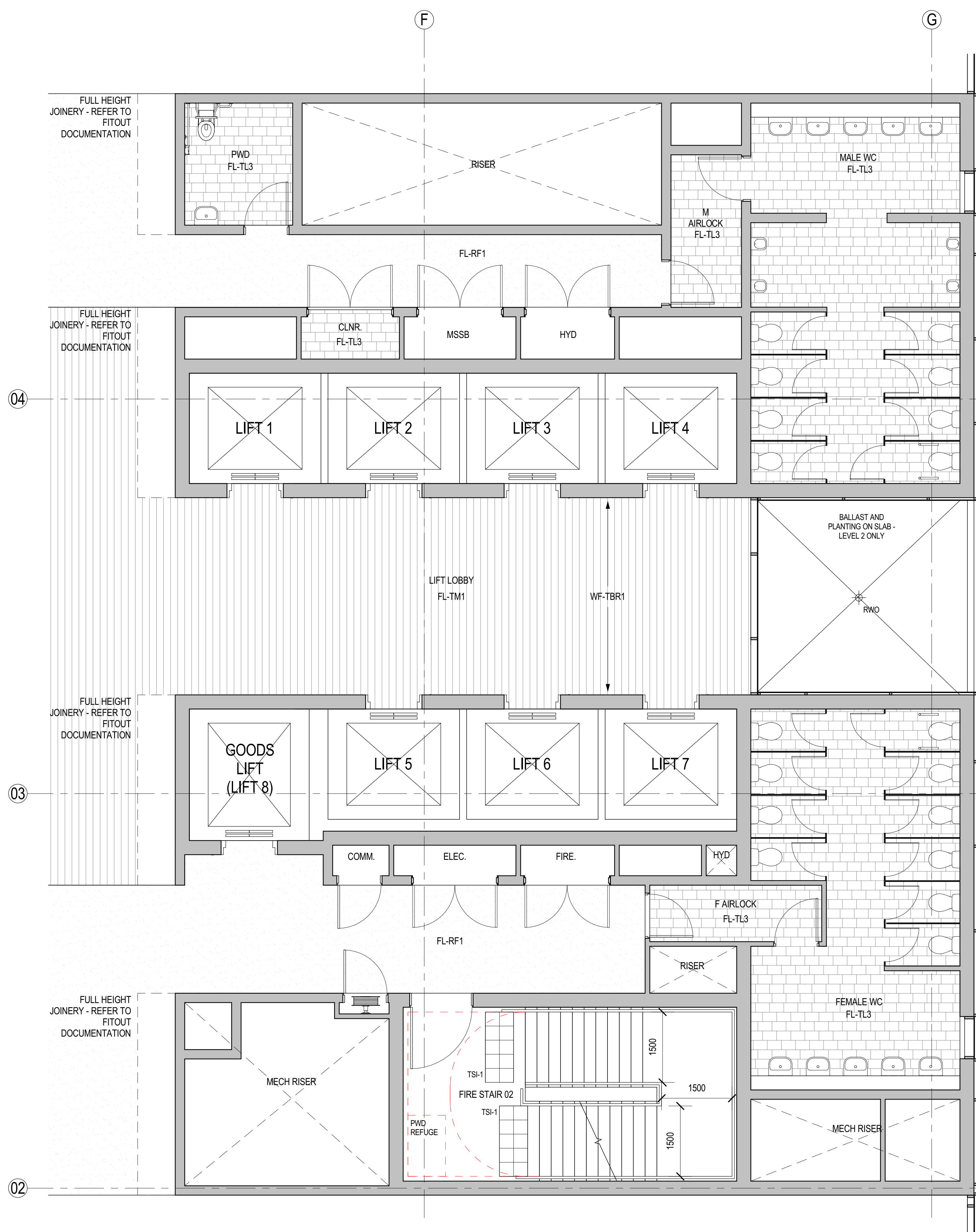
2 TYPICAL CORE - LEVEL 02
