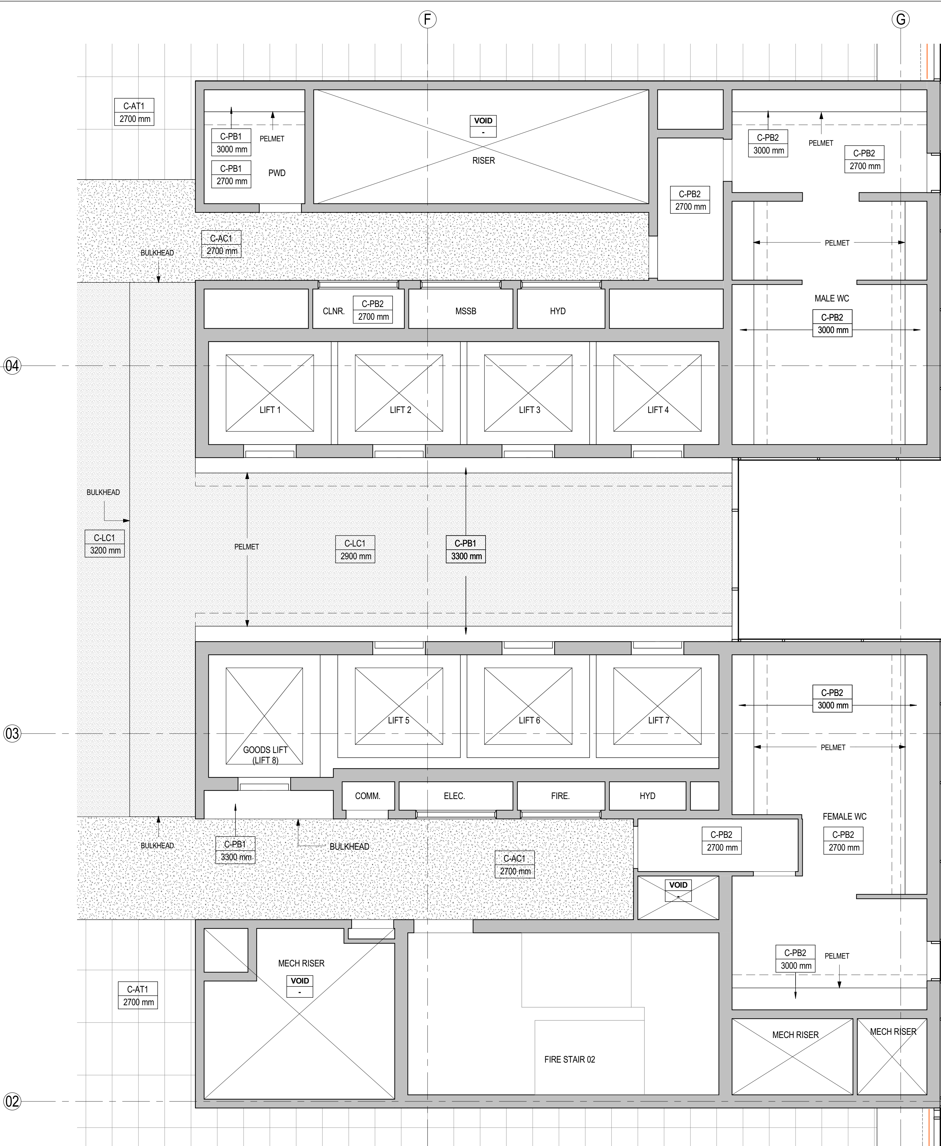
2 RCP - TYPICAL CORE
