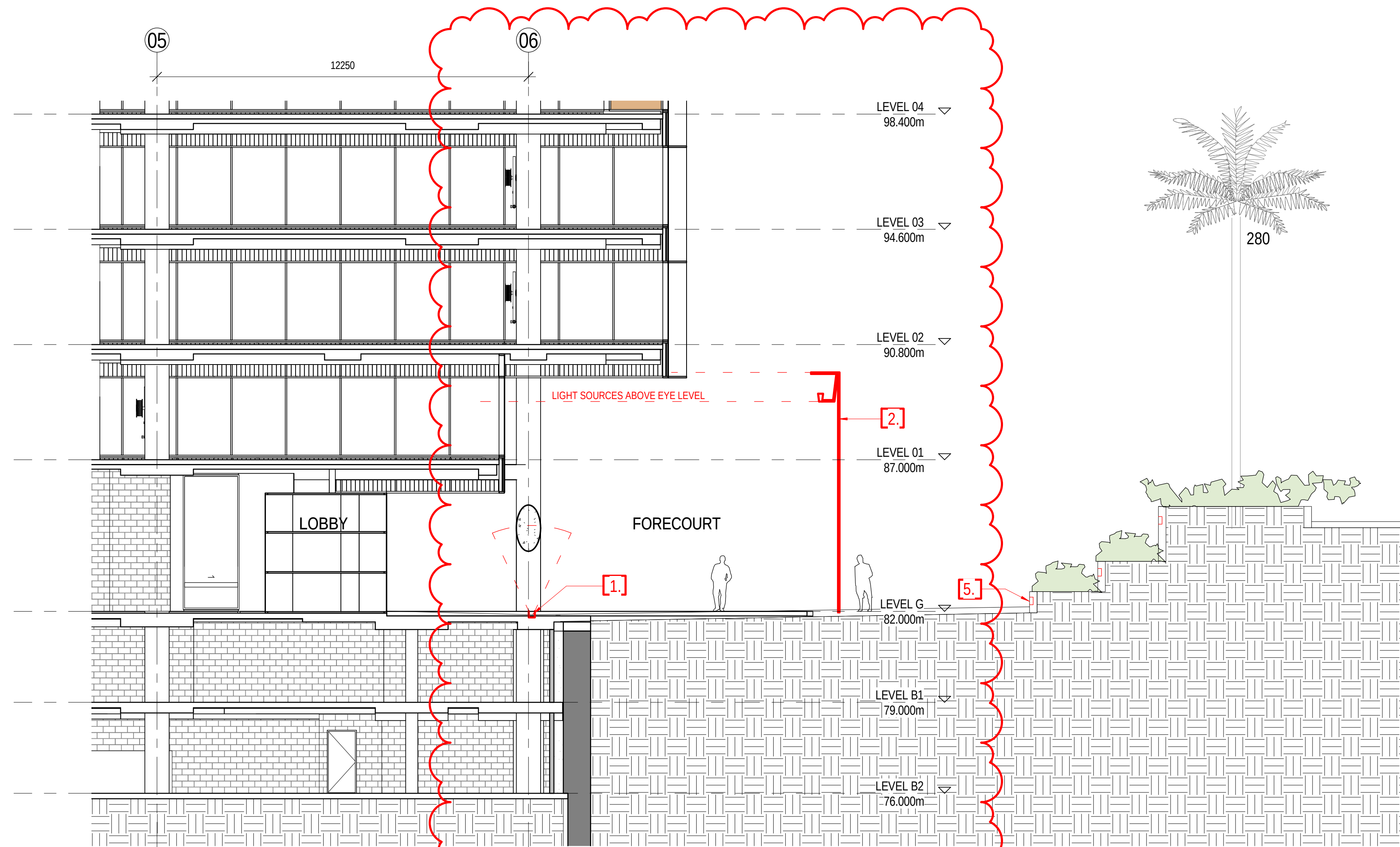
1 SITE SECTION - A
