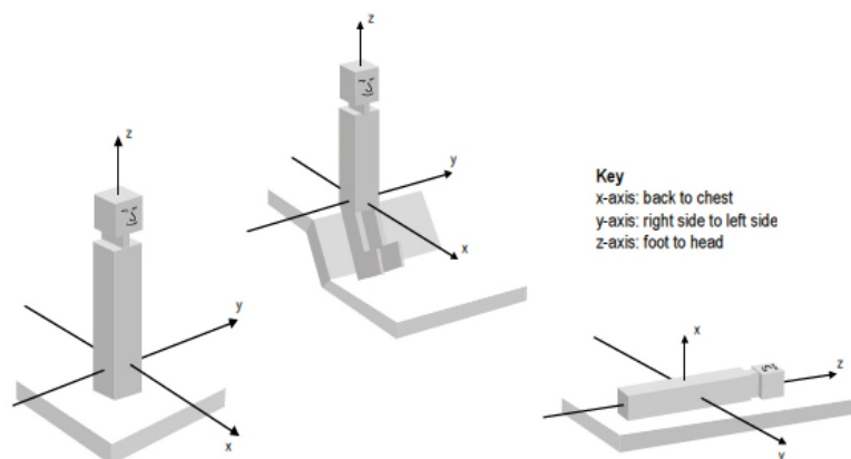
Figure 5 – Orthogonal axes for human exposure to vibration
