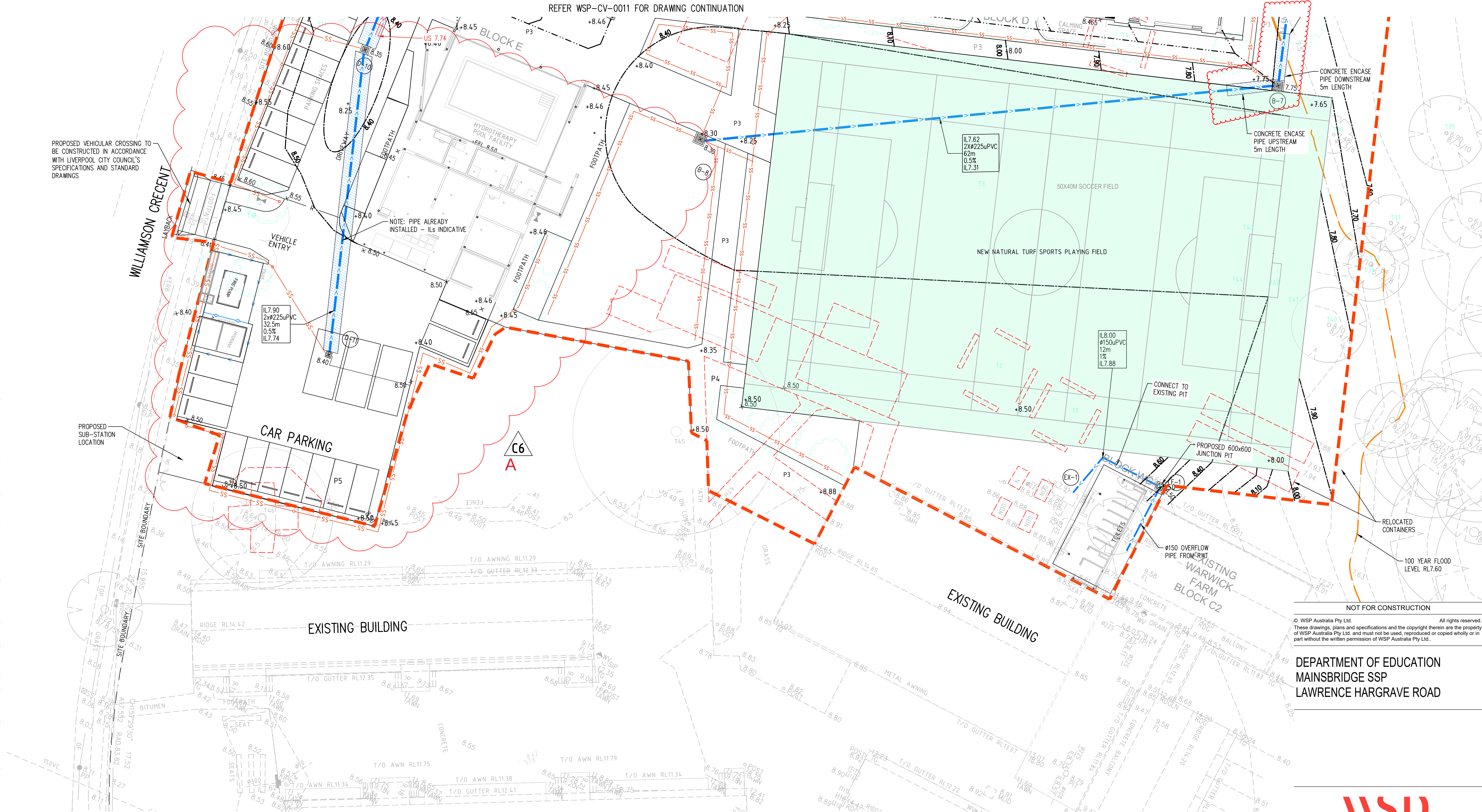
GENERAL ARRANGEMENT PLAN – SHEET 2 OF 2 SCALE: 1:200
