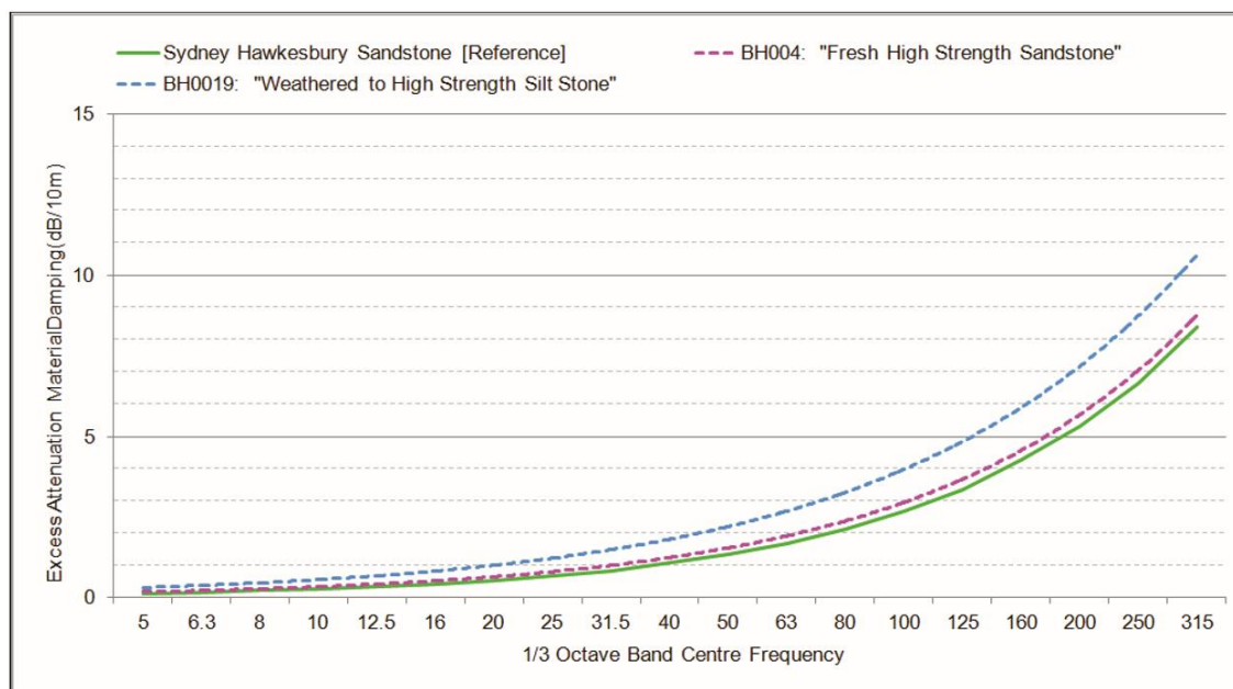
Figure 5-5 Excess material damping (Source: SLR Consulting – Noise and Vibration Technical Paper for Operations and Additional Construction Works)
