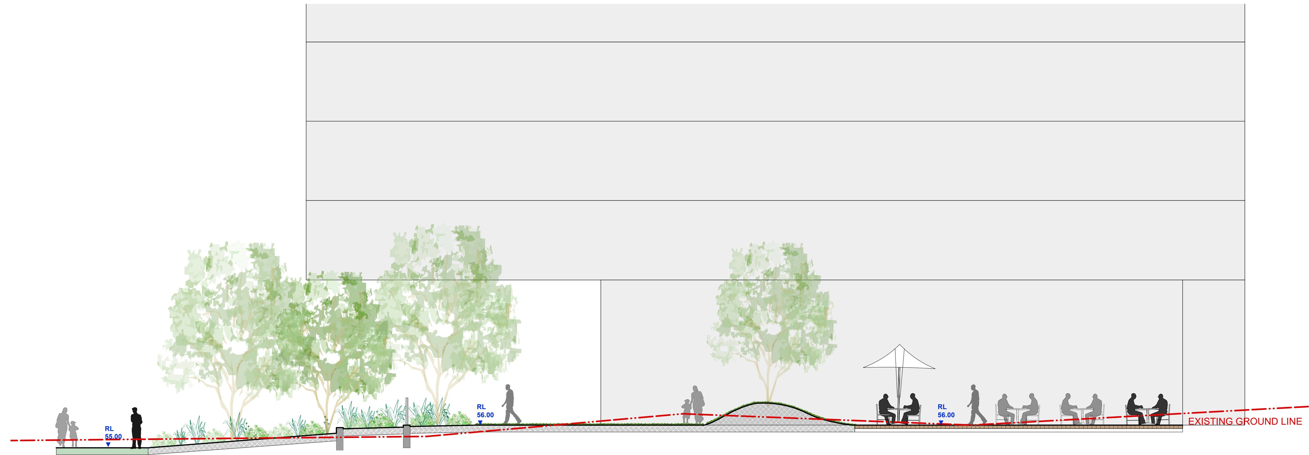
1 SECTION I | RESIDENTIAL COURTYARD Scale 1:100
