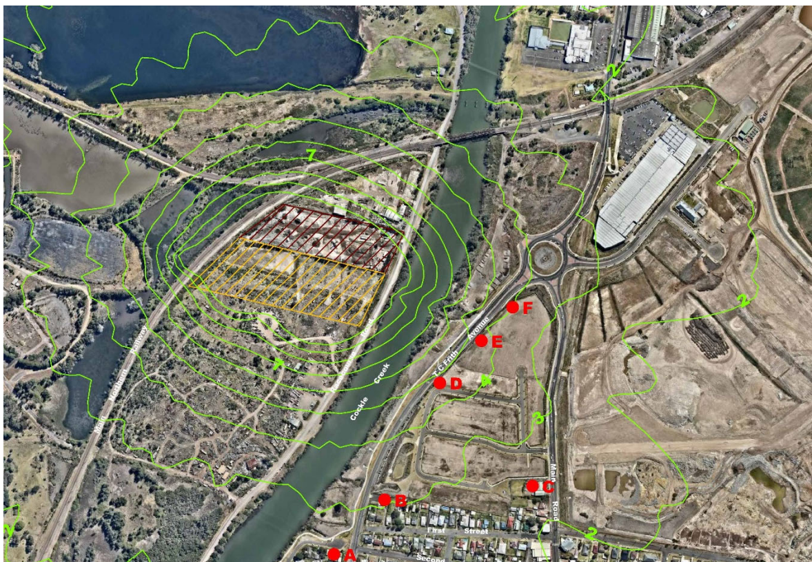
Figure 3 Dust modelling results - PM 2.5 dust component (criterion 25µg/m 3 , ● indicates receptor position).
