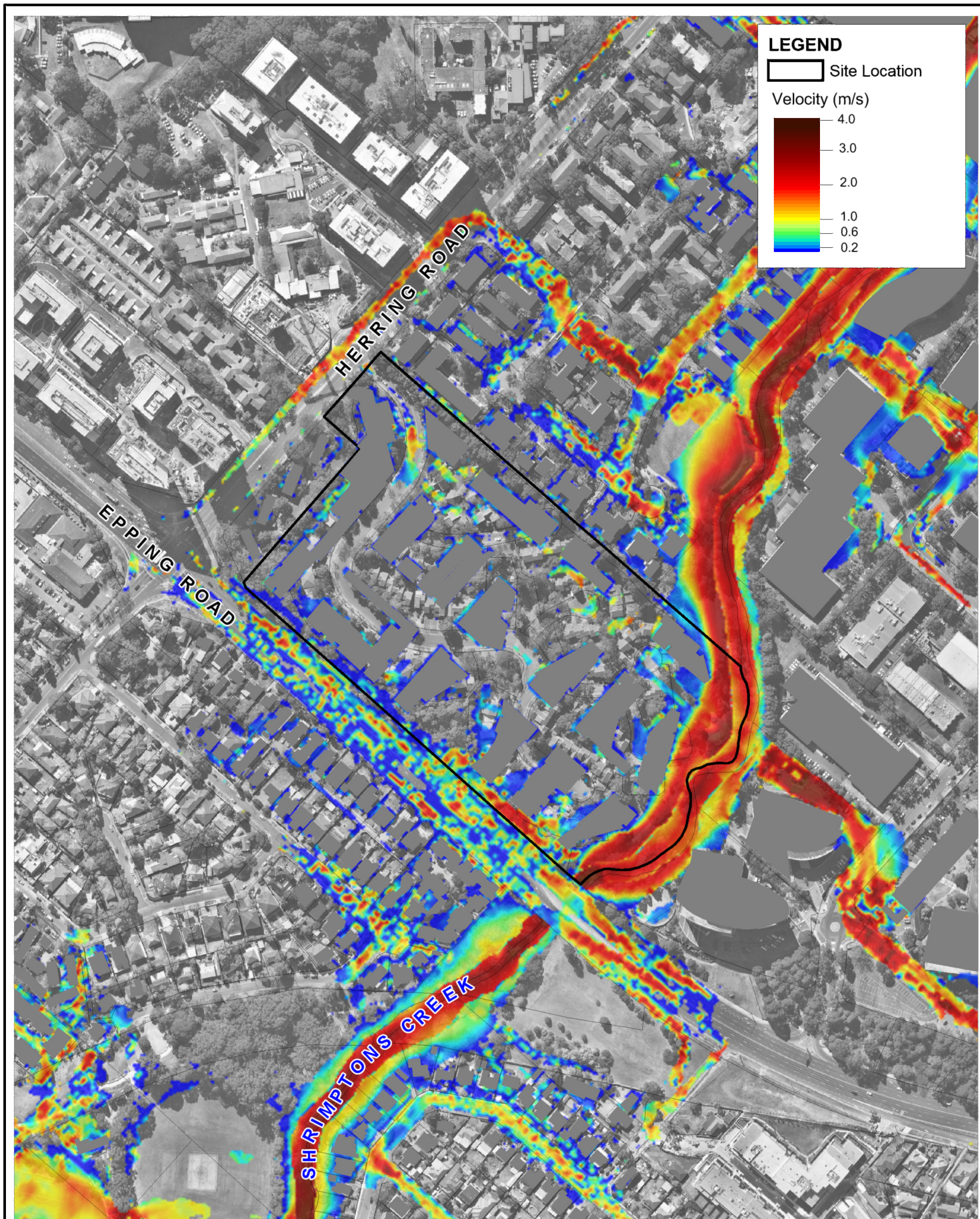
Title: Peak Flood Velocity - Developed Scenario Probable Maximum Flood (PMF)
