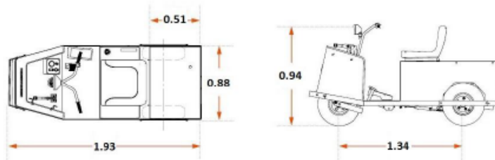
Figure 11: Schematic of a Typical Electric Ride On Tug Device
