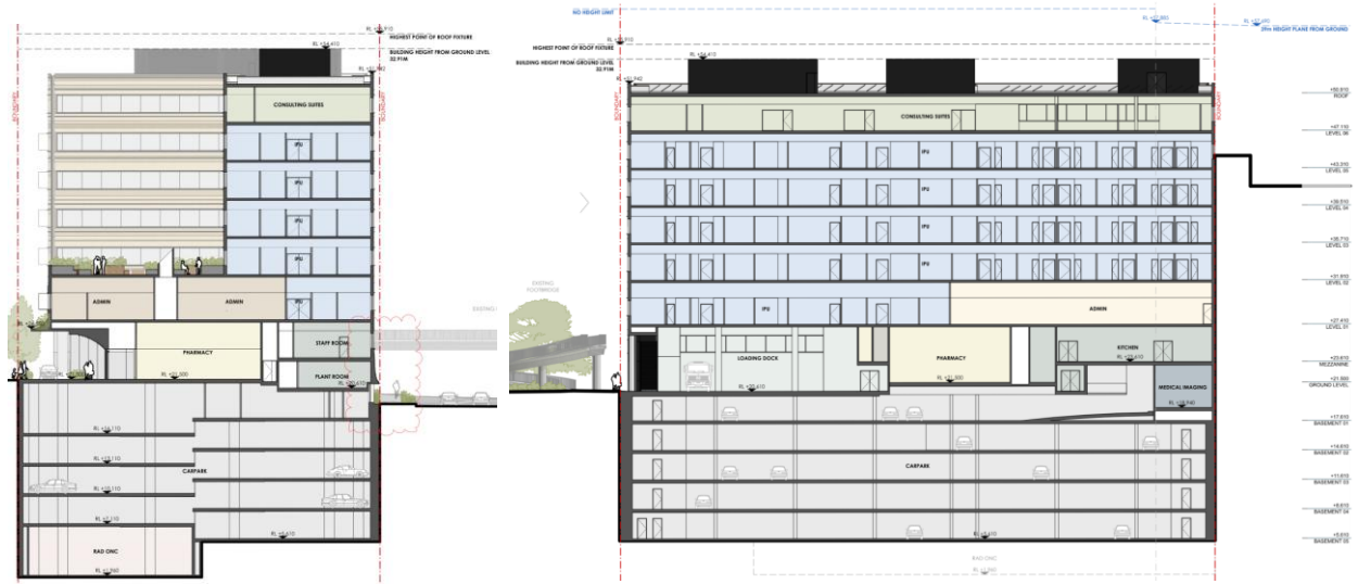
Figure 1-4: Proposed Sections - Clinical Tower Site
