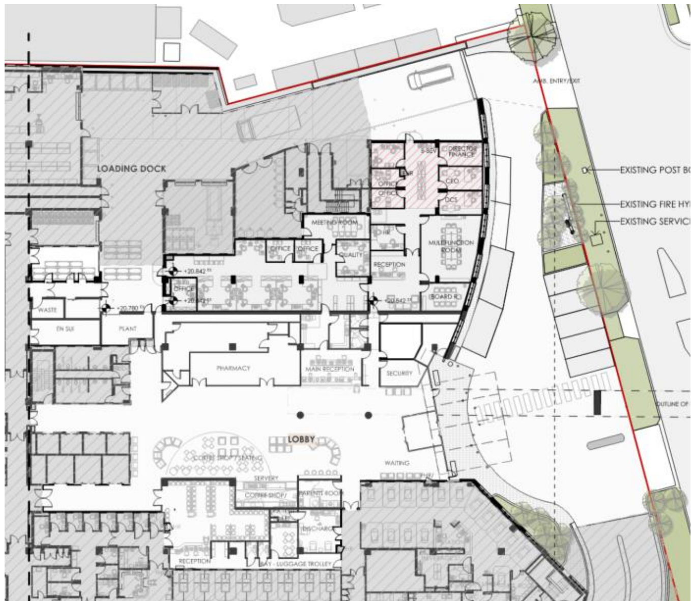
Figure 1-5: Proposed Floor Plan - Main Hospital Campus
