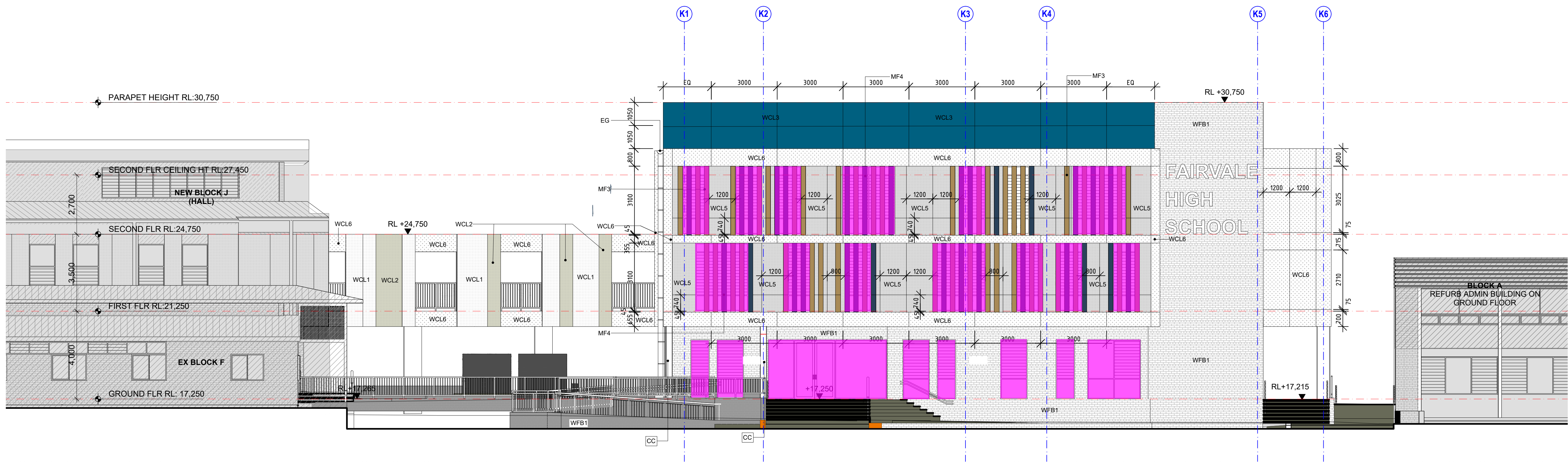
BLOCK K - SOUTH ELEVATION 1:100
