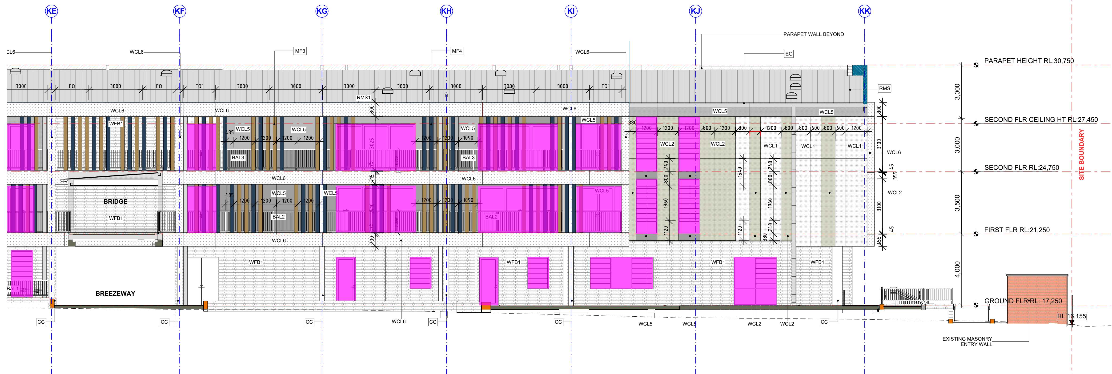
BLOCK K - WEST ELEVATION 1:100
