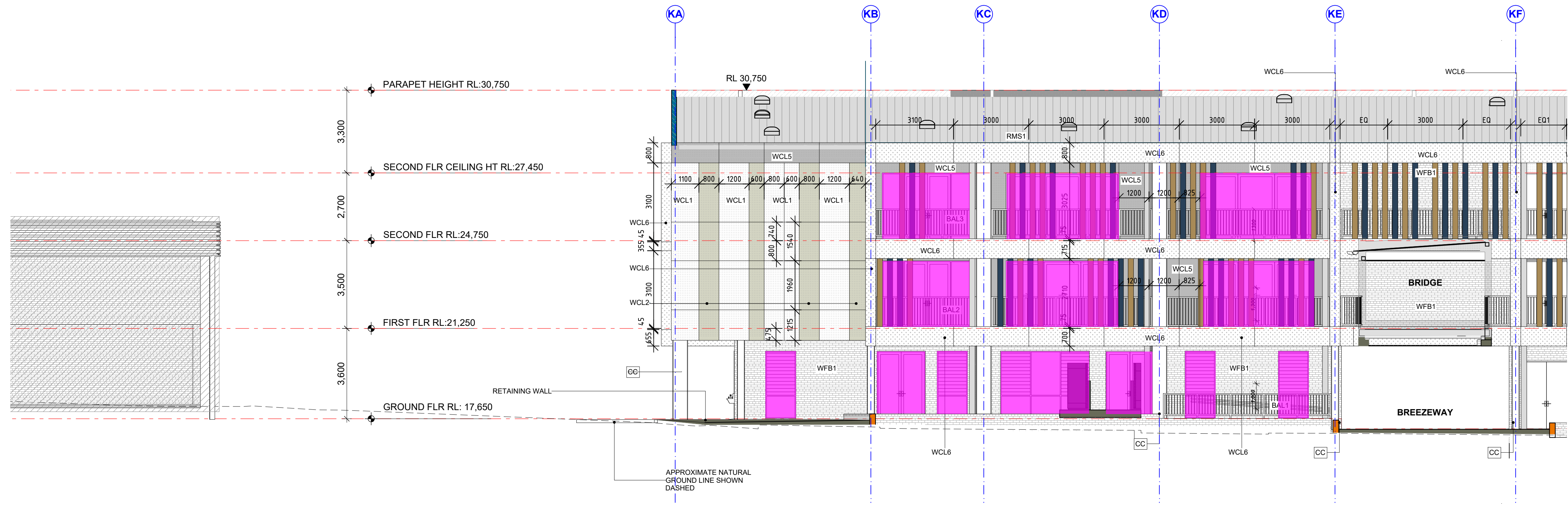
BLOCK K - WEST ELEVATION 1:100
