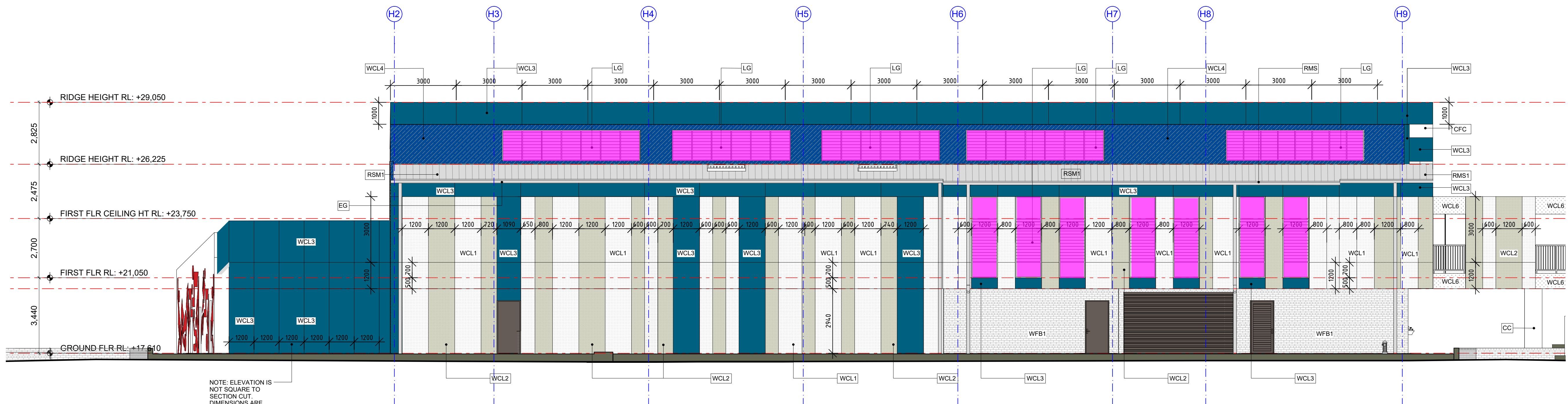
1 BLOCK J - HALL BUILDING - SOUTH ELEVATION 1:100
