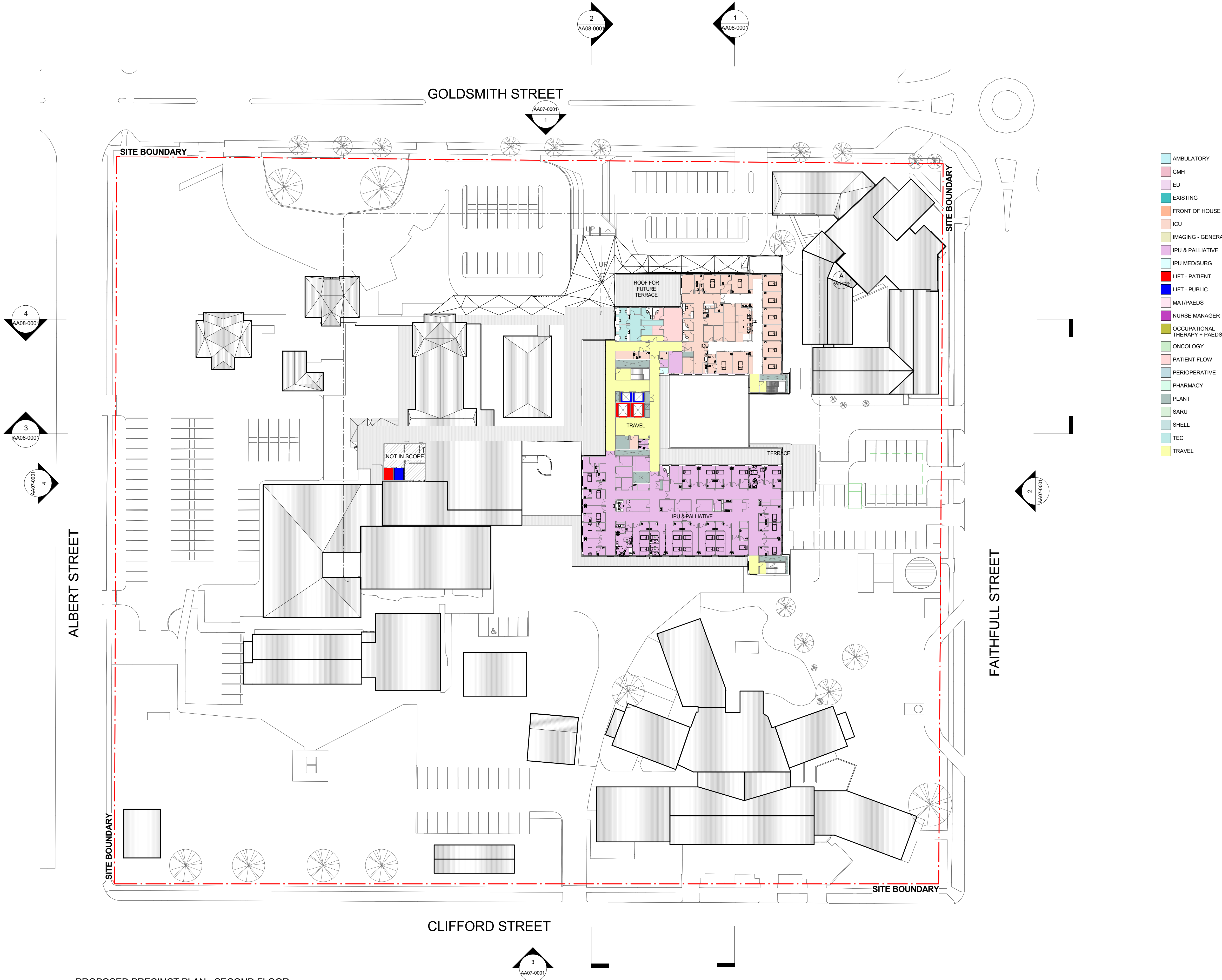
1 PROPOSED PRECINCT PLAN - SECOND FLOOR 1 : 500
