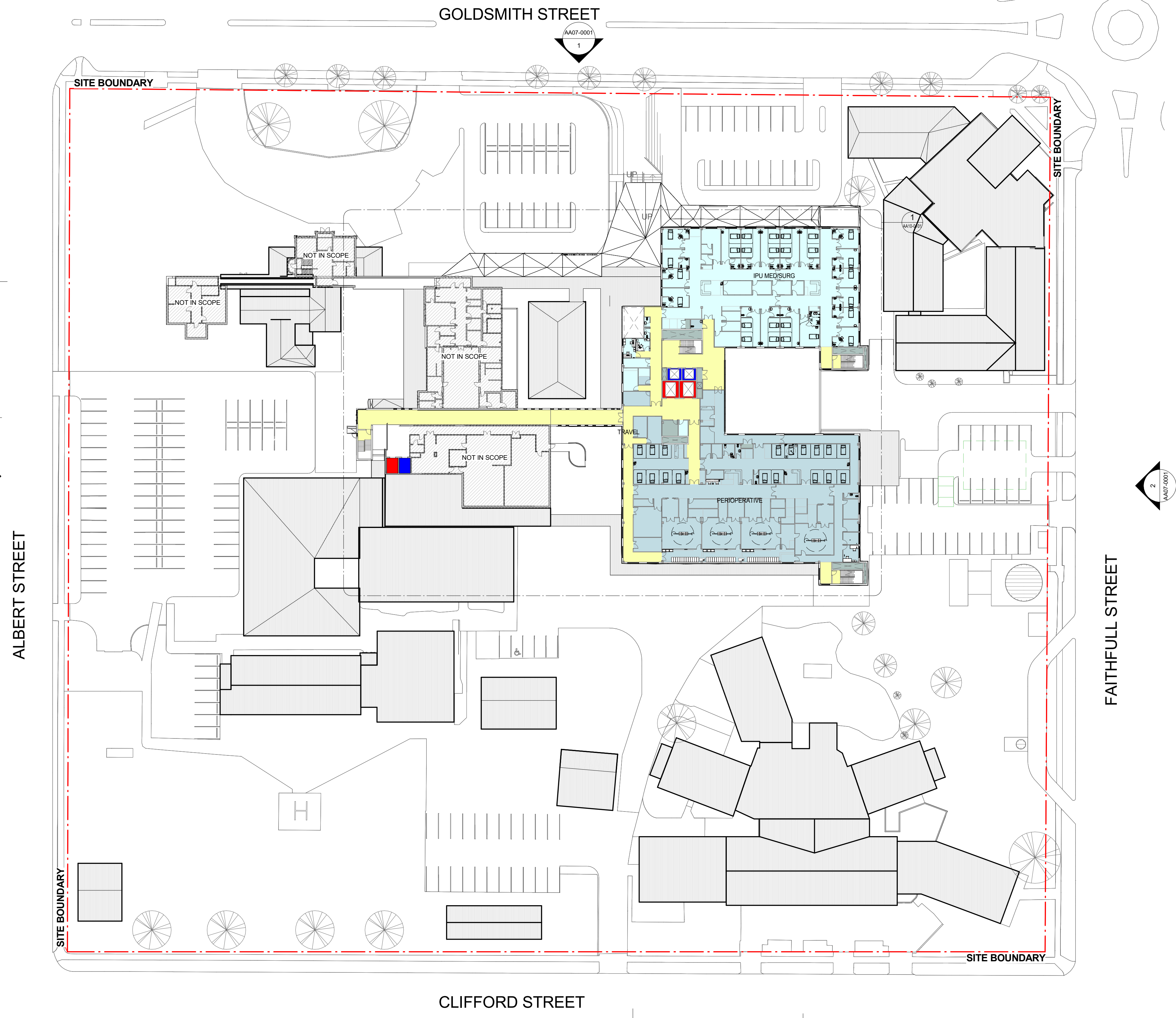
1 PROPOSED PRECINCT PLAN - FIRST FLOOR 1:500
