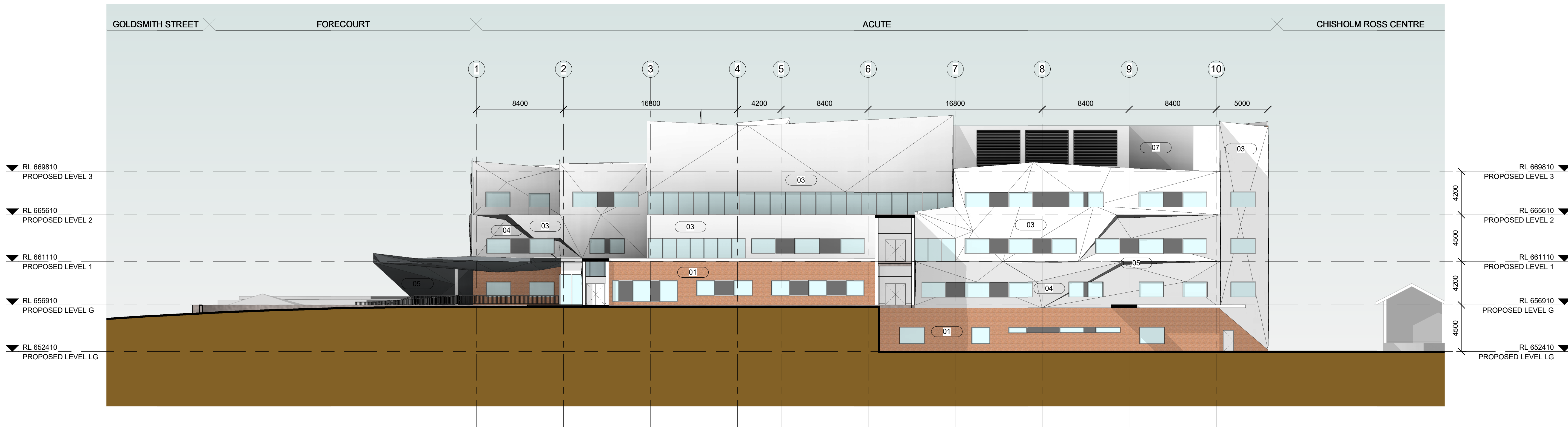
1 ELEVATION - PROPOSED - WEST 1:200
