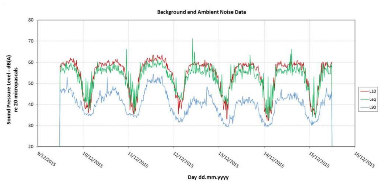
Figure 4: Long term noise monitoring results at location L4-background noise measurement
