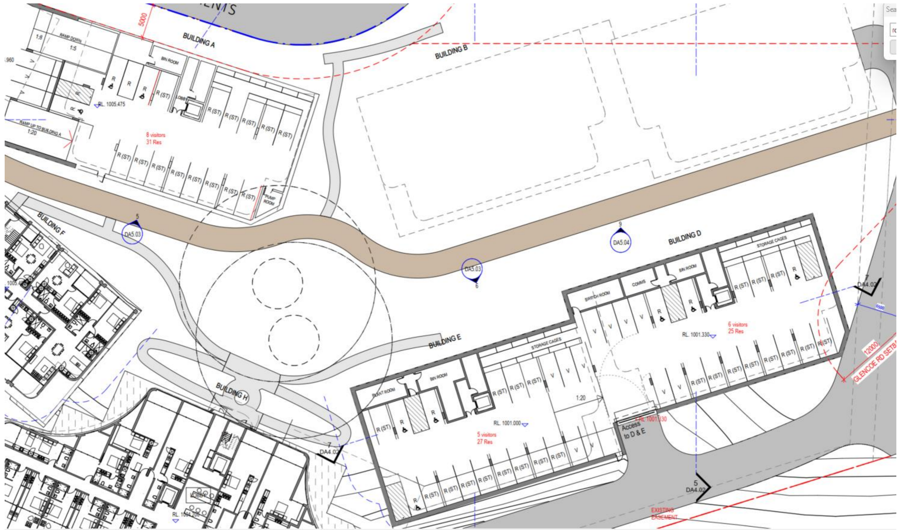
Source: Antoniades Architects, Ground Floor Plan, Rev E, 17/10/2025
