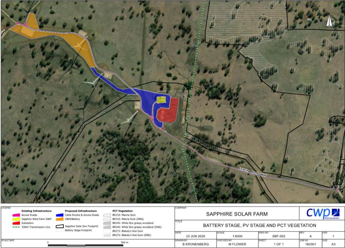
Figure 1-2 Stage 1 Project layout
