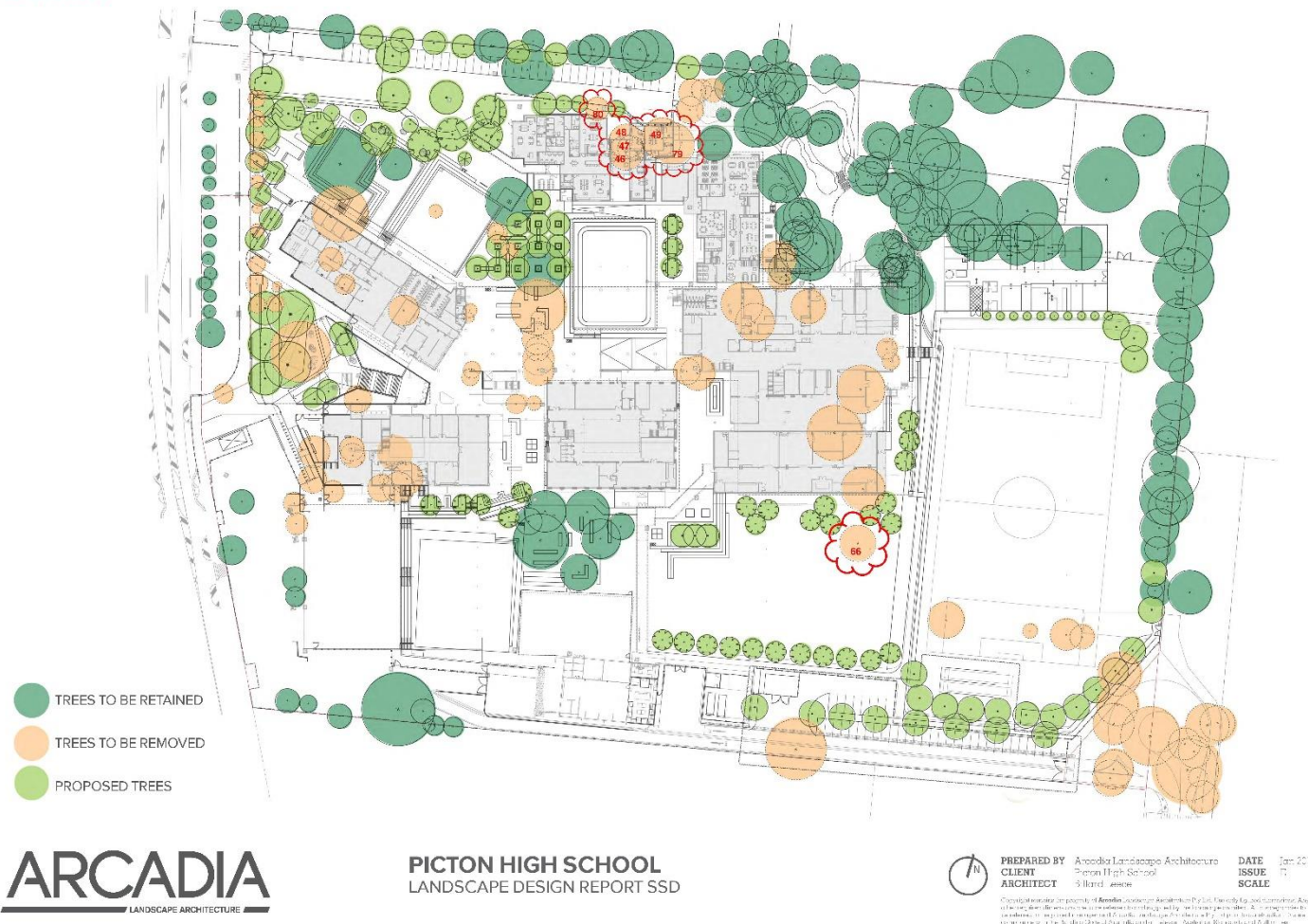
Figure 1: Tree retention and removal plan.
