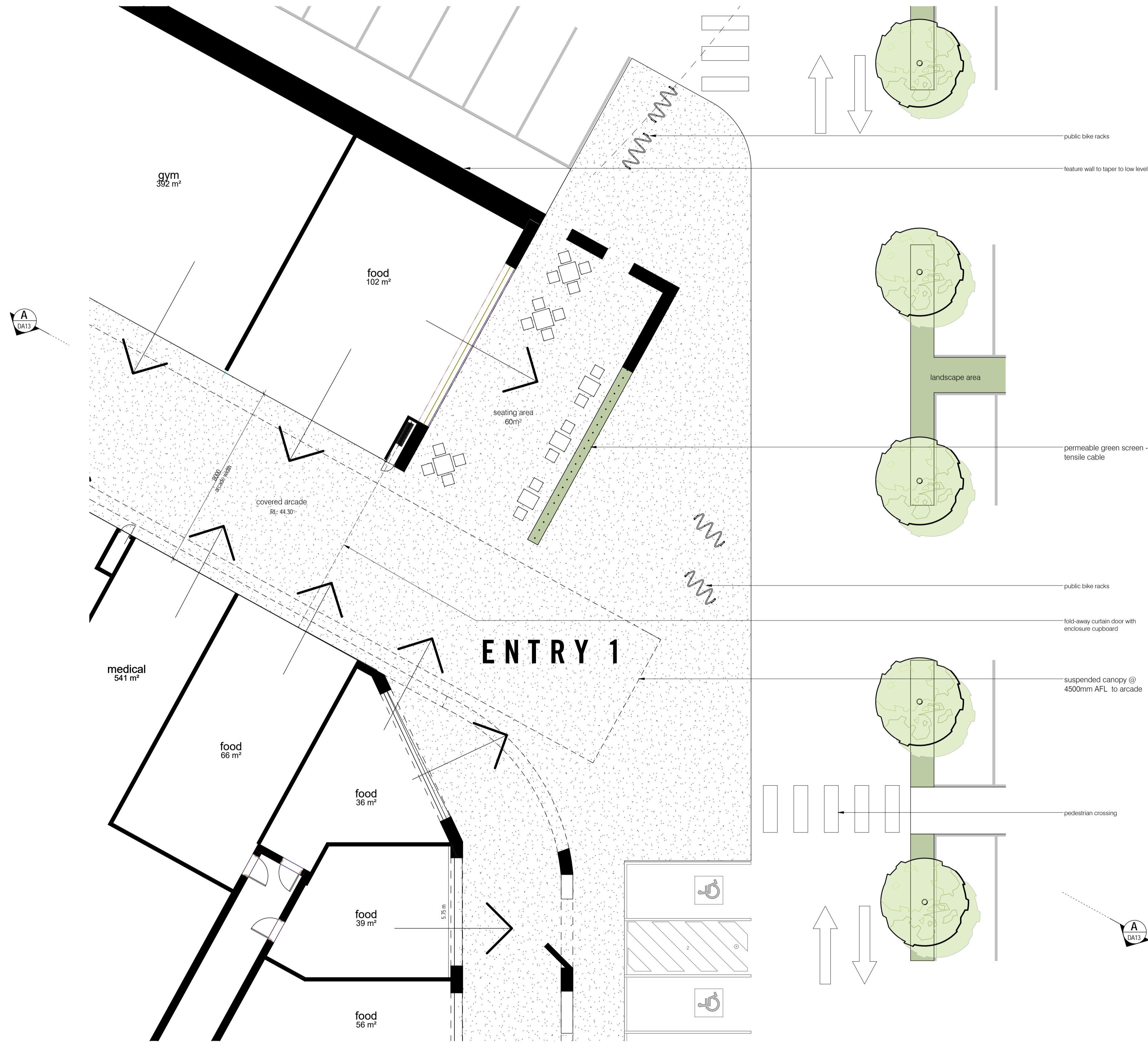
PROPOSED ZONE A PLAN (ENTRY 1) 1 : 100
