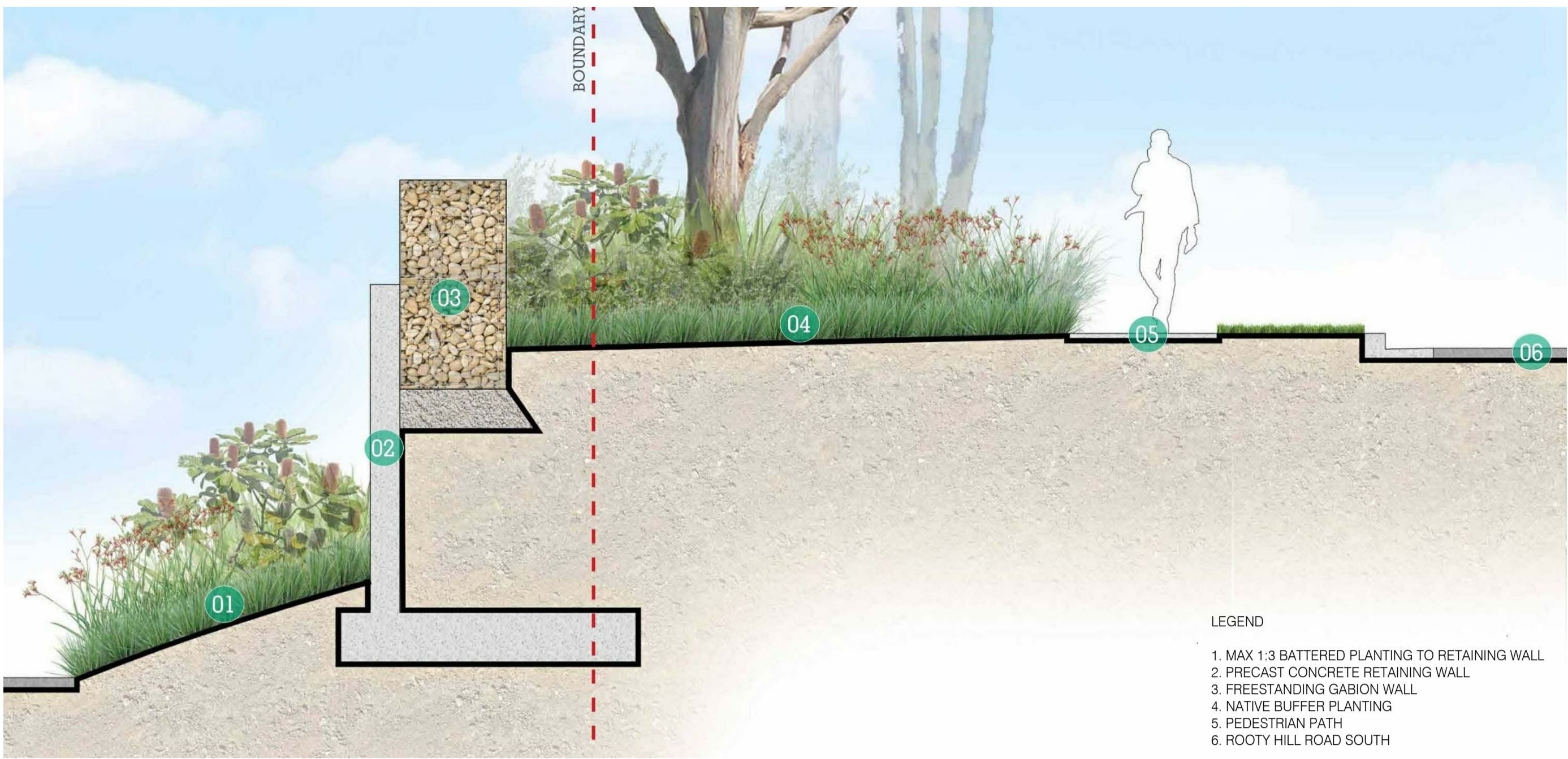
5 Screening Section 1:10
