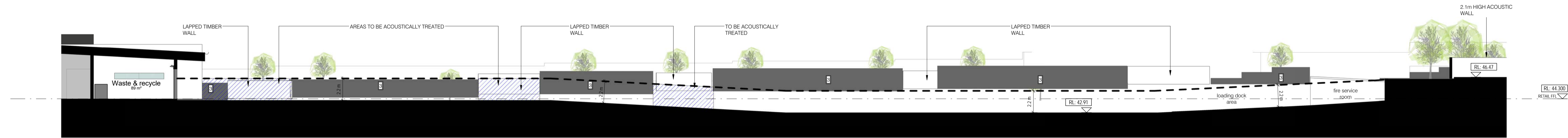
STAGE 1 - BOH SECTION 1:200
