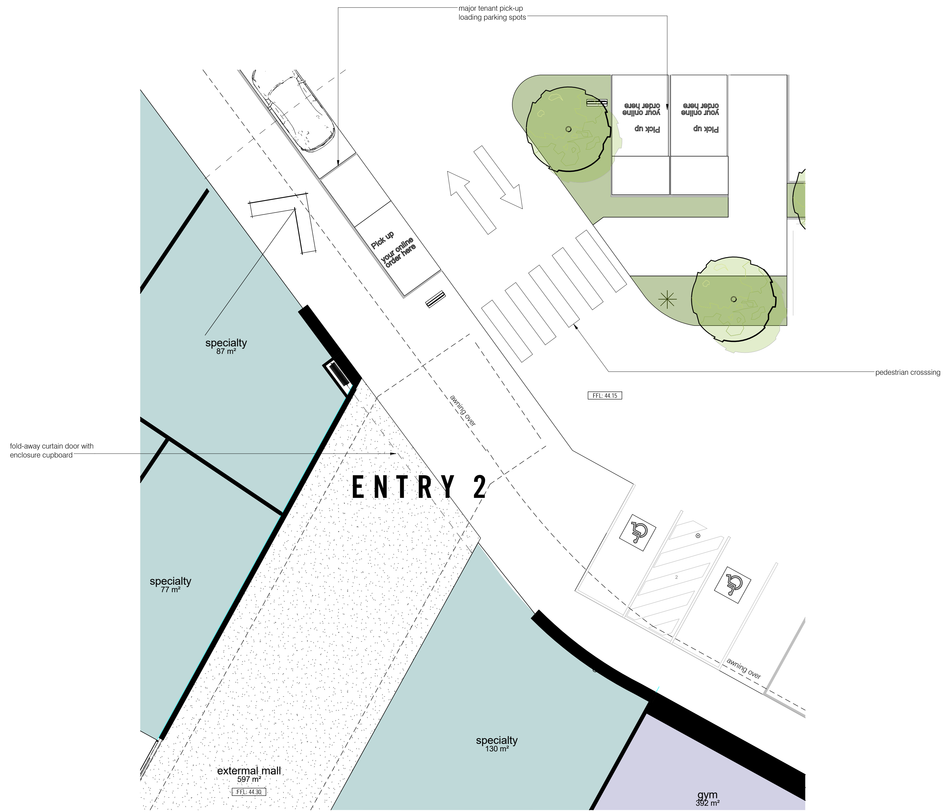
PROPOSED ZONE B PLAN (ENTRY 2) 1 : 100
