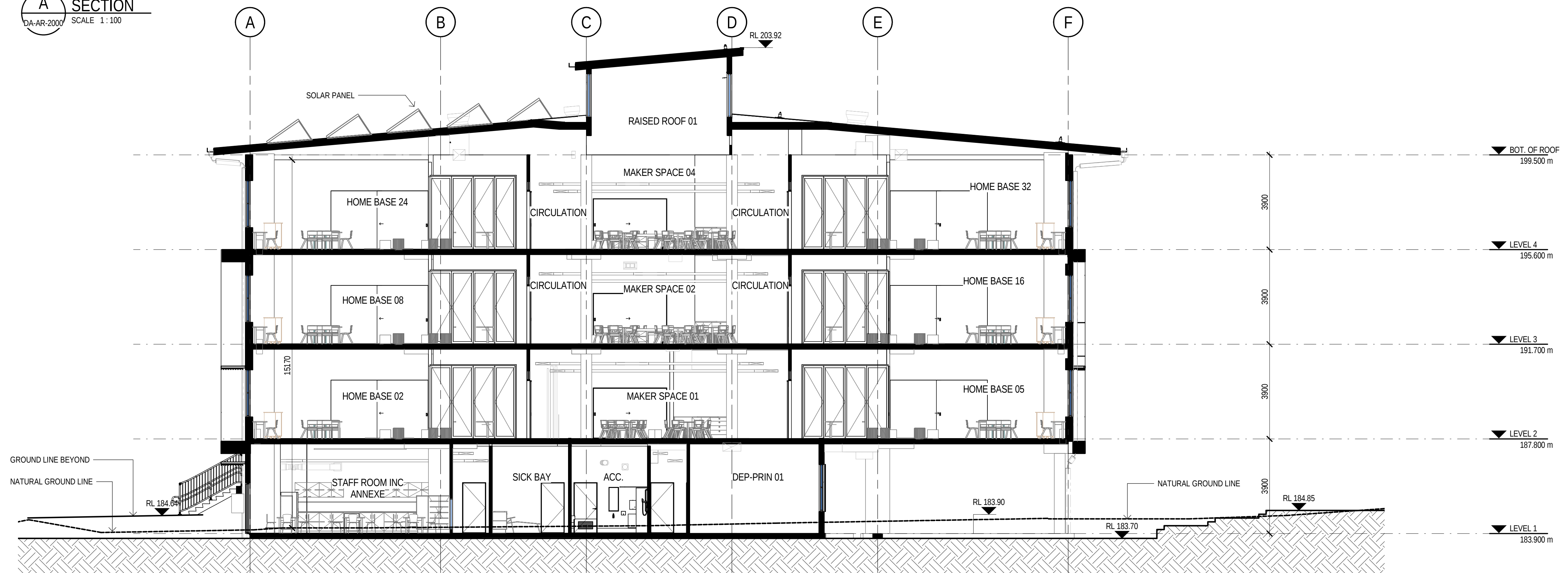
B SECTION DA-AR-2000 SCALE 1:100
