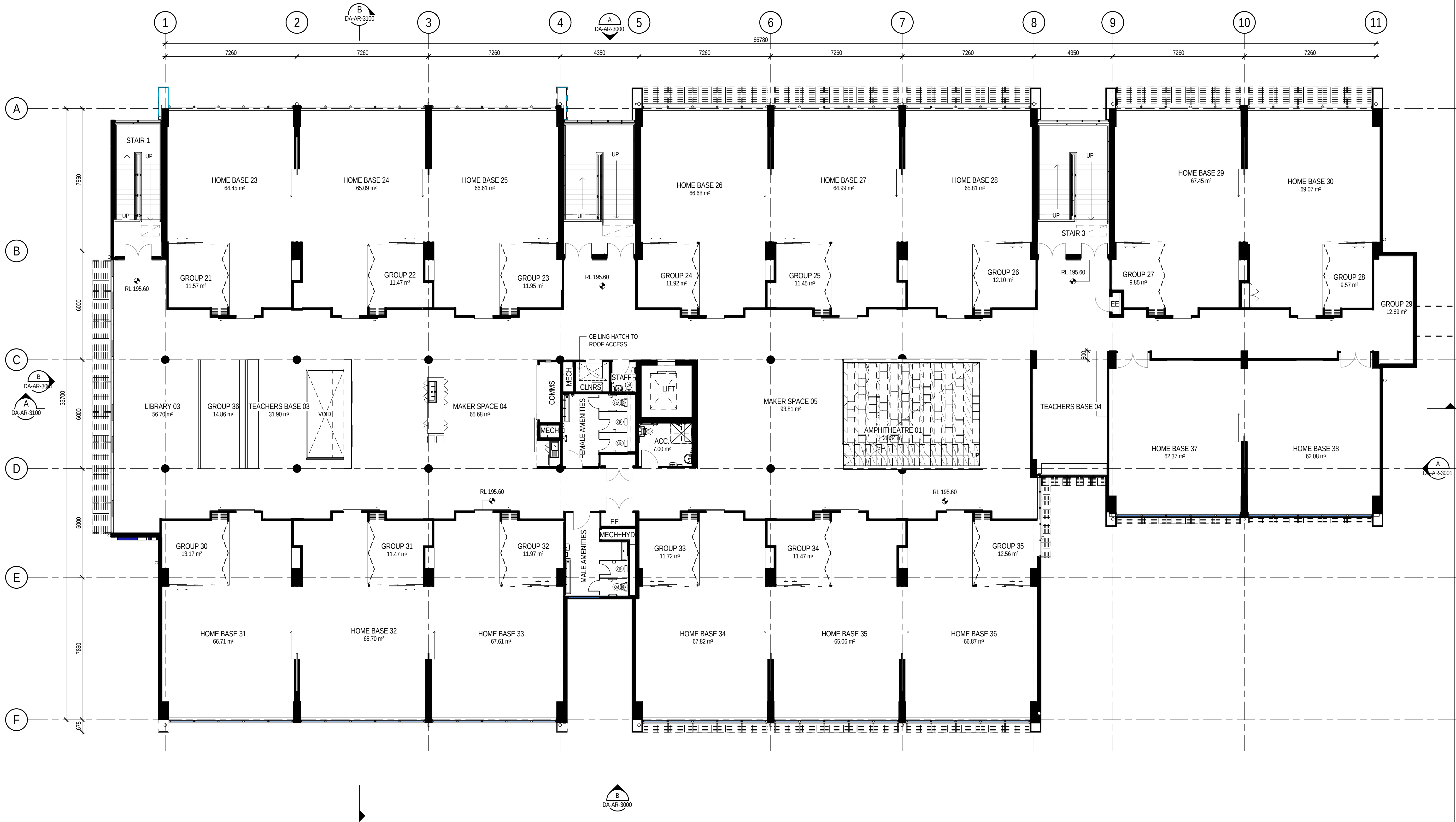
GENERAL ARRANGEMENT - LEVEL 4 SCALE 1:100
