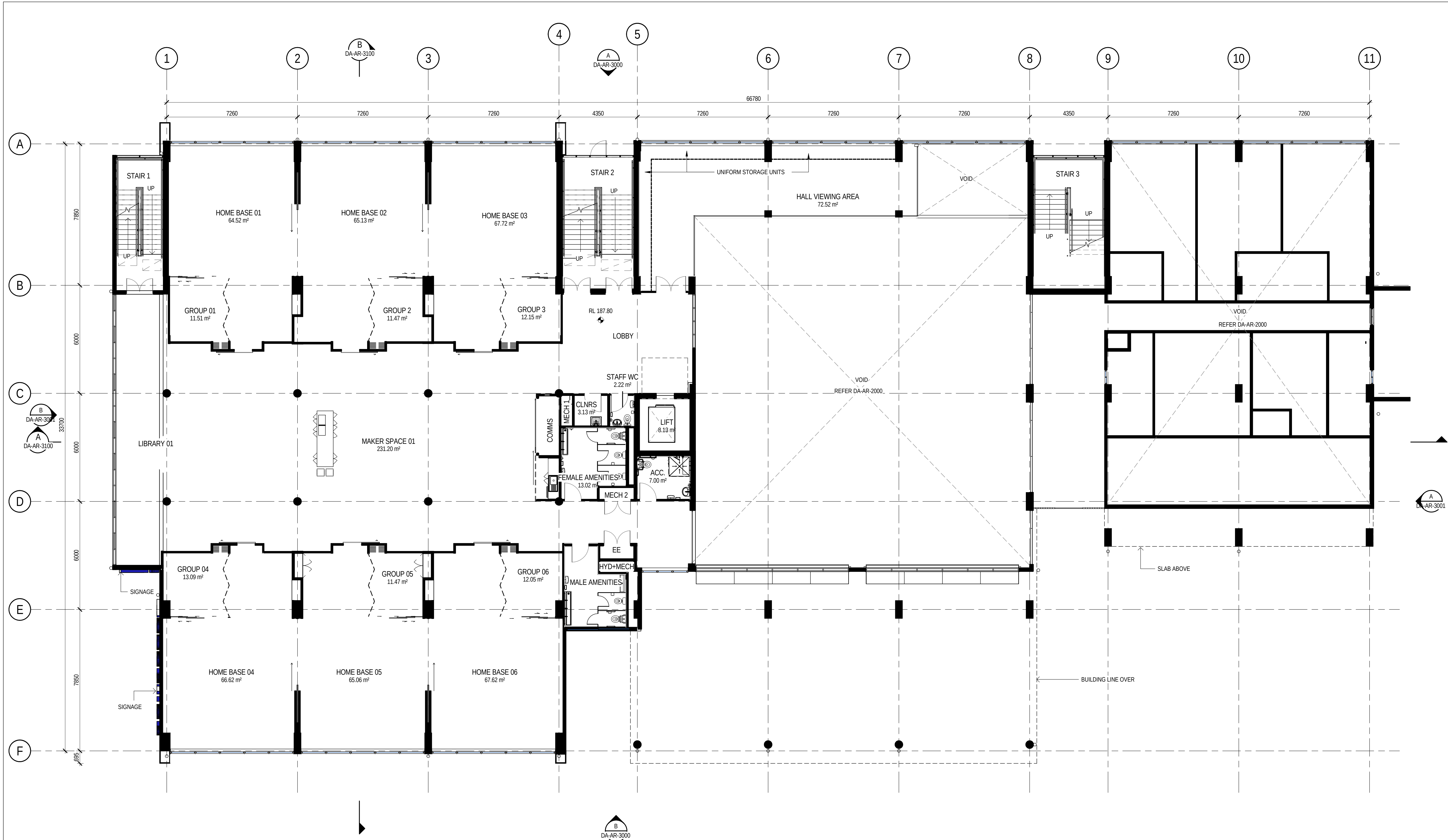
GENERAL ARRANGEMENT - LEVEL 2 SCALE 1:100
