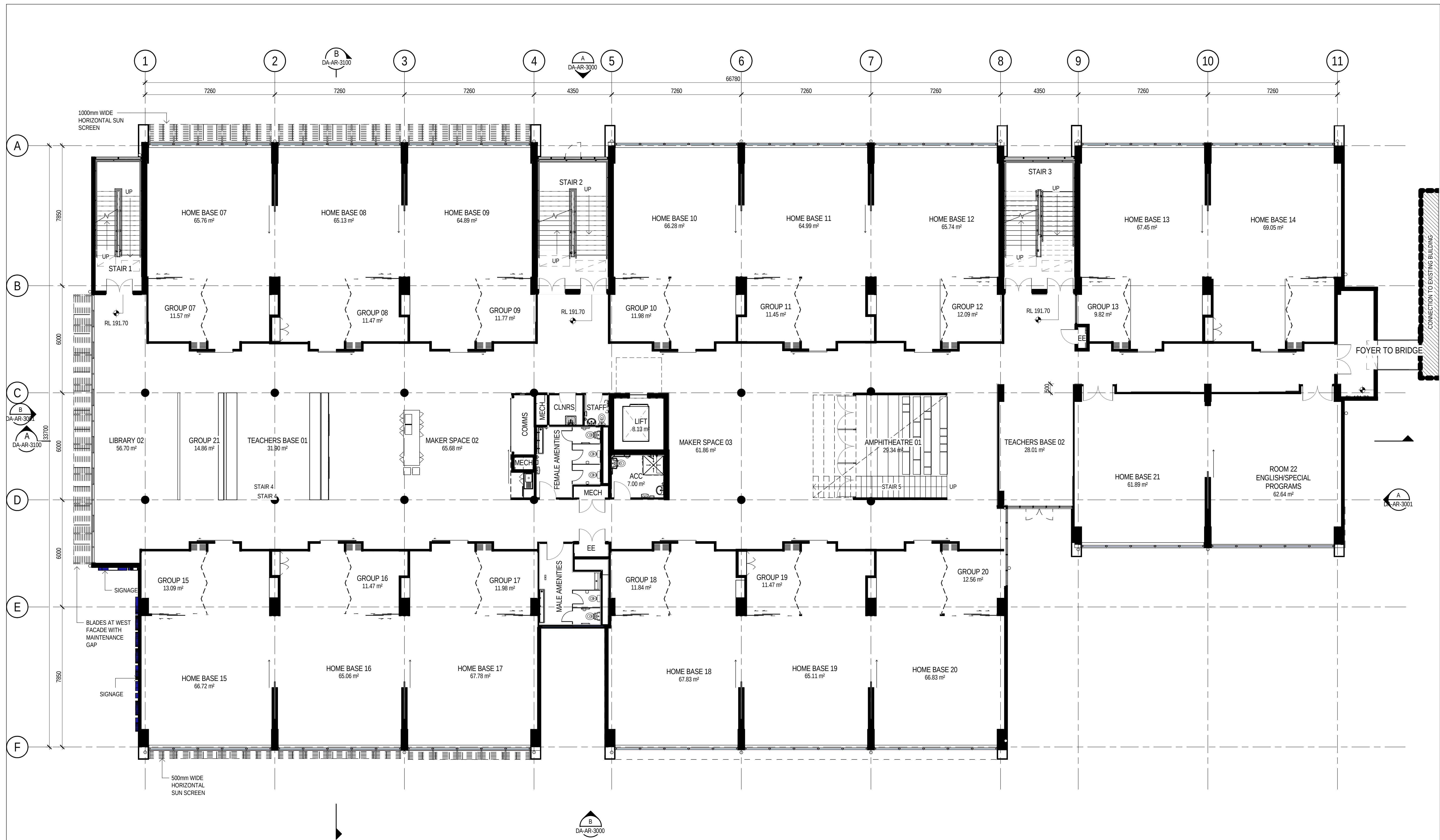
GENERAL ARRANGEMENT - LEVEL 3 SCALE 1:100
