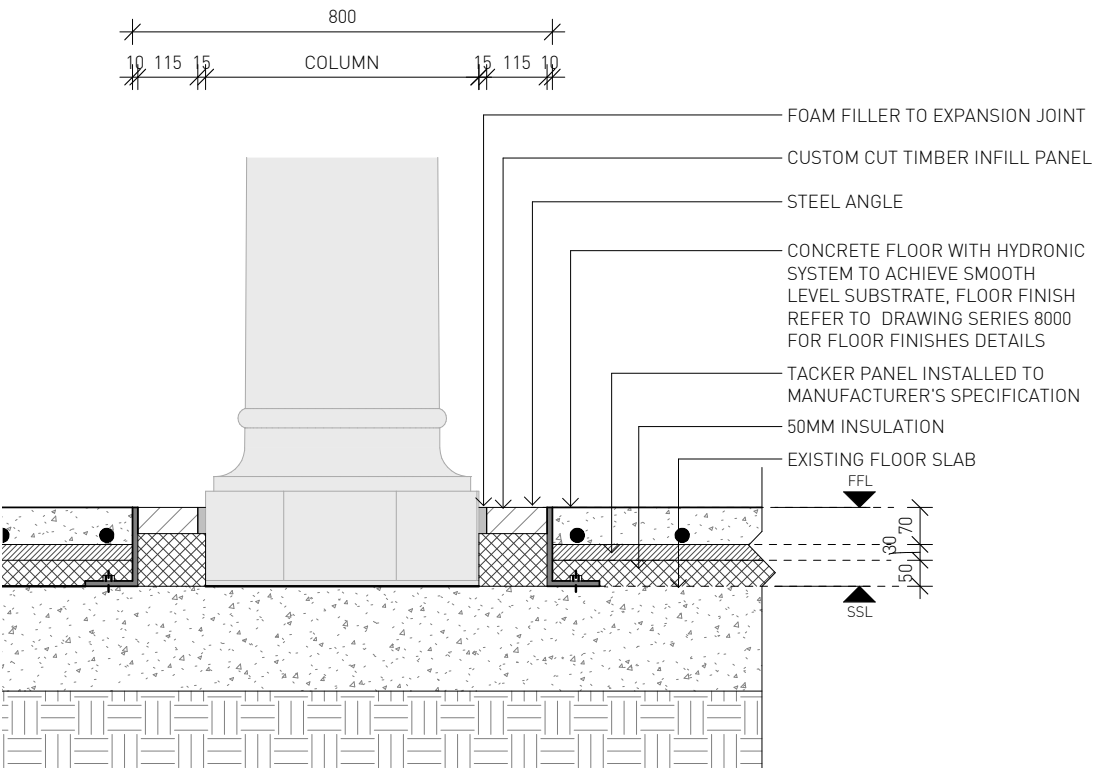
Ground Floor Bays 1-4A Circulation Zones Floor Build Up Detail
