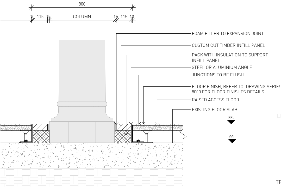
Ground Floor Bays 5-13 Floor Build Up Detail
