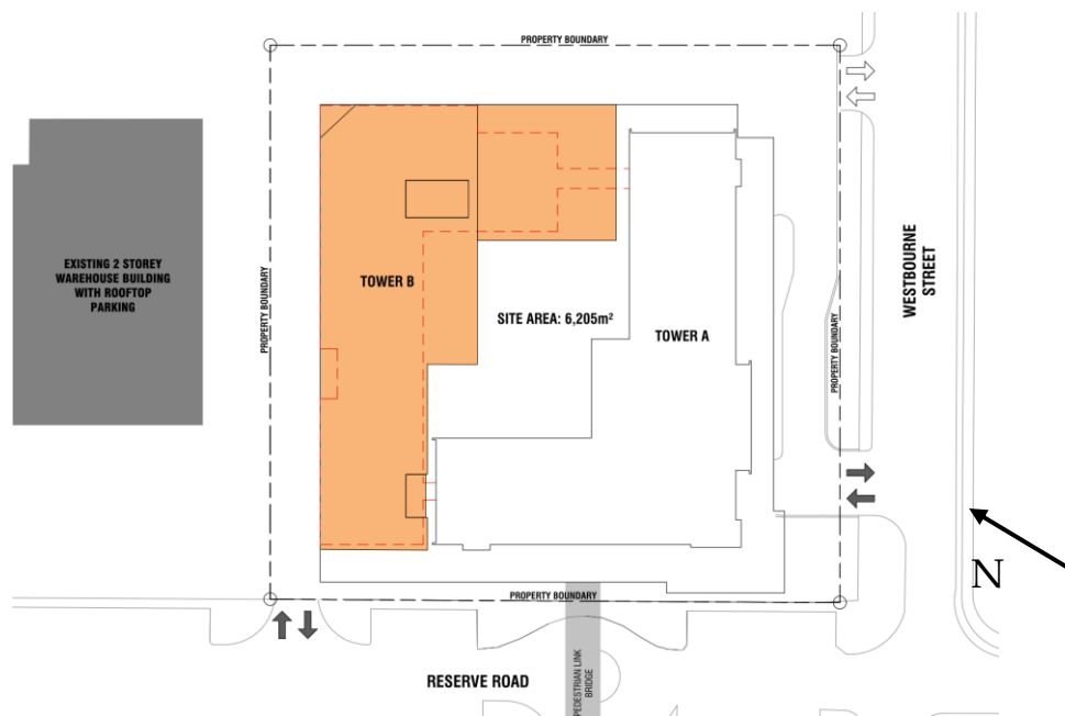
Figure 7: Site plan showing Tower B envelope
