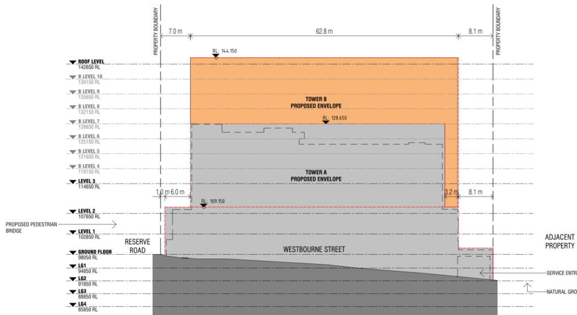
Figure 8: South elevation of proposed development
