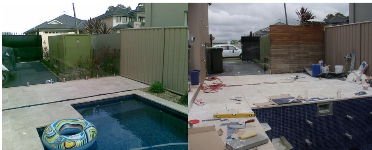
Before and After. This swimming pool in Endeavour Energy's network area at Middleton Grange NSW had to be modified to comply with the restriction for the padmount substation on the use of land in relation to swimming pools.
