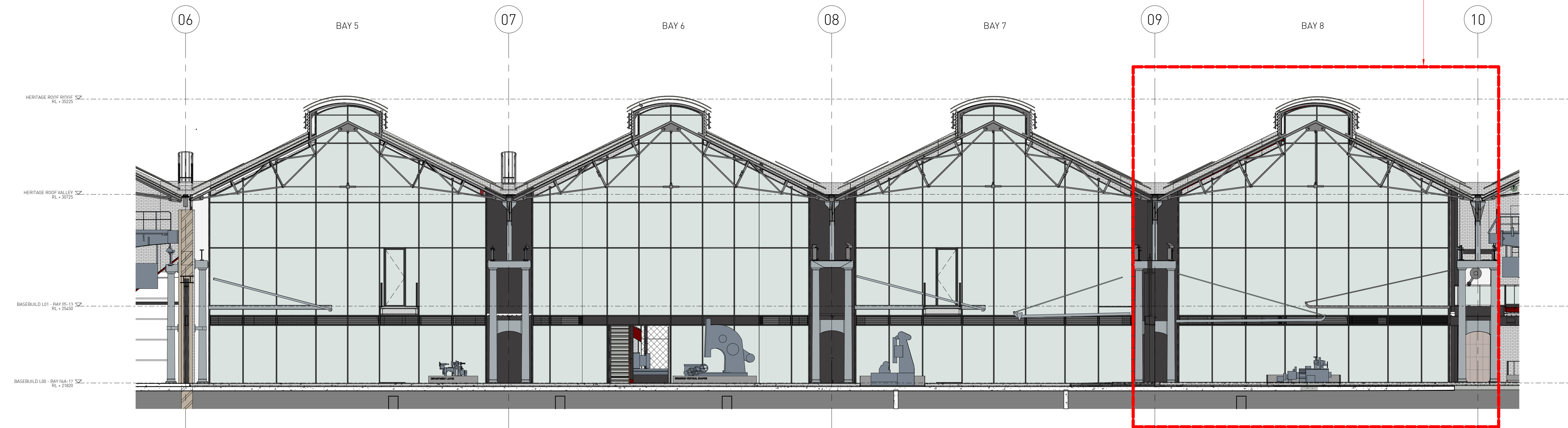
2 FULL HEIGHT GLAZING ELEVATION - BAYS 5-8 SOUTH 1 : 100
