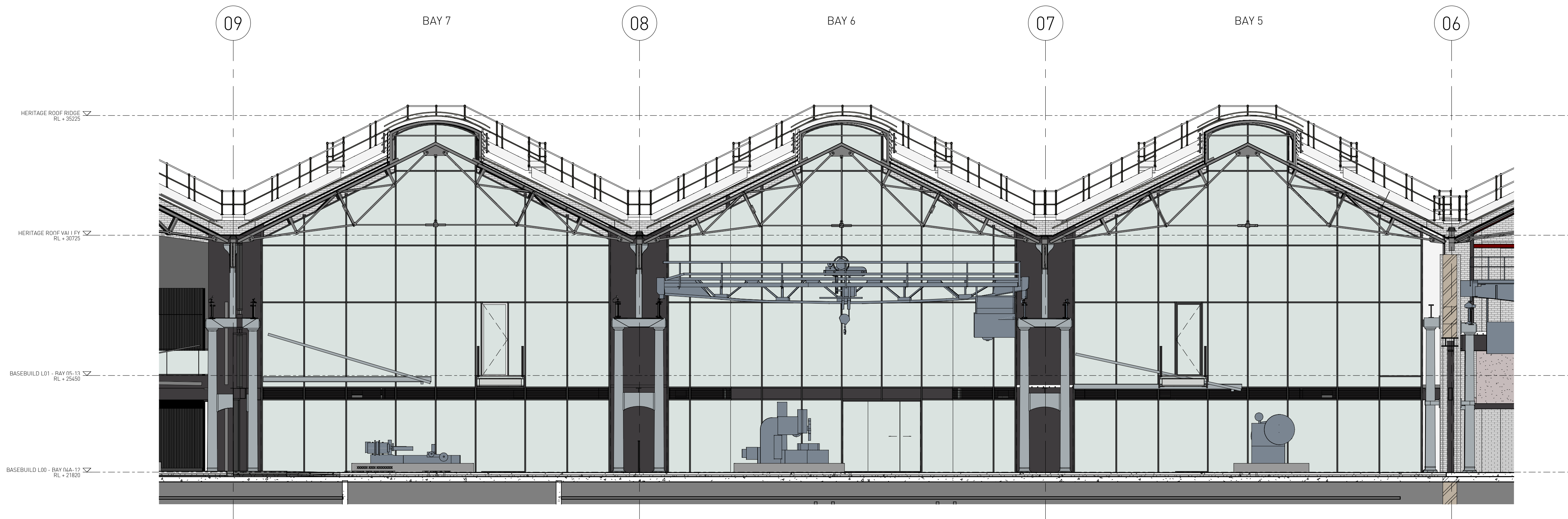
1 FULL HEIGHT GLAZING ELEVATION - BAYS 5-7 NORTH 1 : 100
