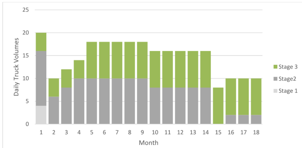
Figure 6: Daily Cumulative Truck Volumes for Construction Stages 1 - 3
