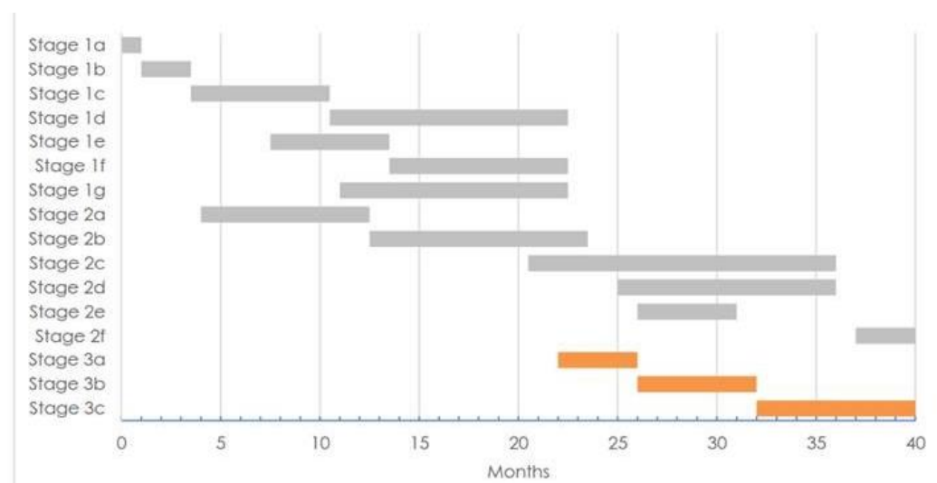
Figure 4: Projected construction schedule for Building 1, Building 2, Building 3 and the Locomotive Workshop
