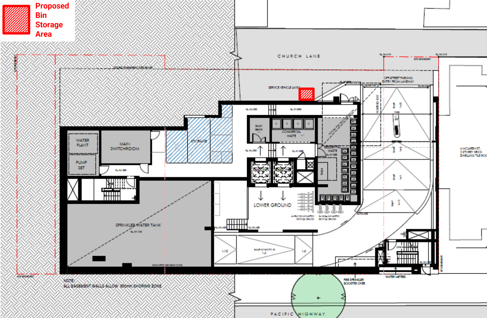
Source: nettletontribe, Drawing No. 14344_DA105A, Issue 1, June 2025 - Lower Ground Floor Plan
