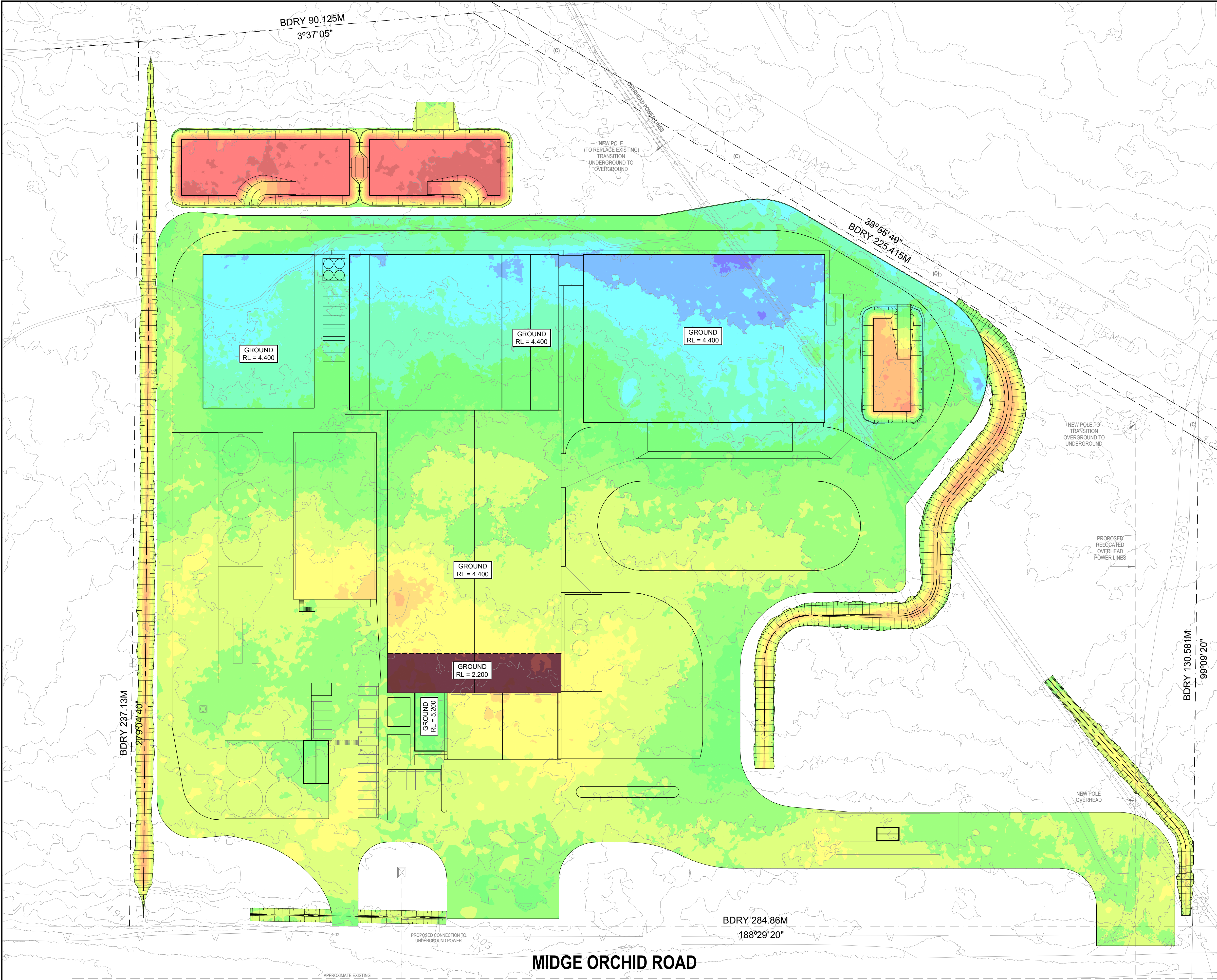
BULK EARTHWORKS PLAN 1:500
