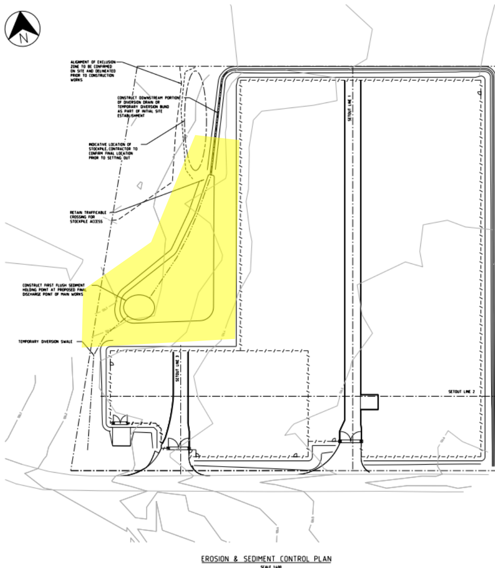
Figure 17 Evaporation Pond (highlighted in YELLOW)
