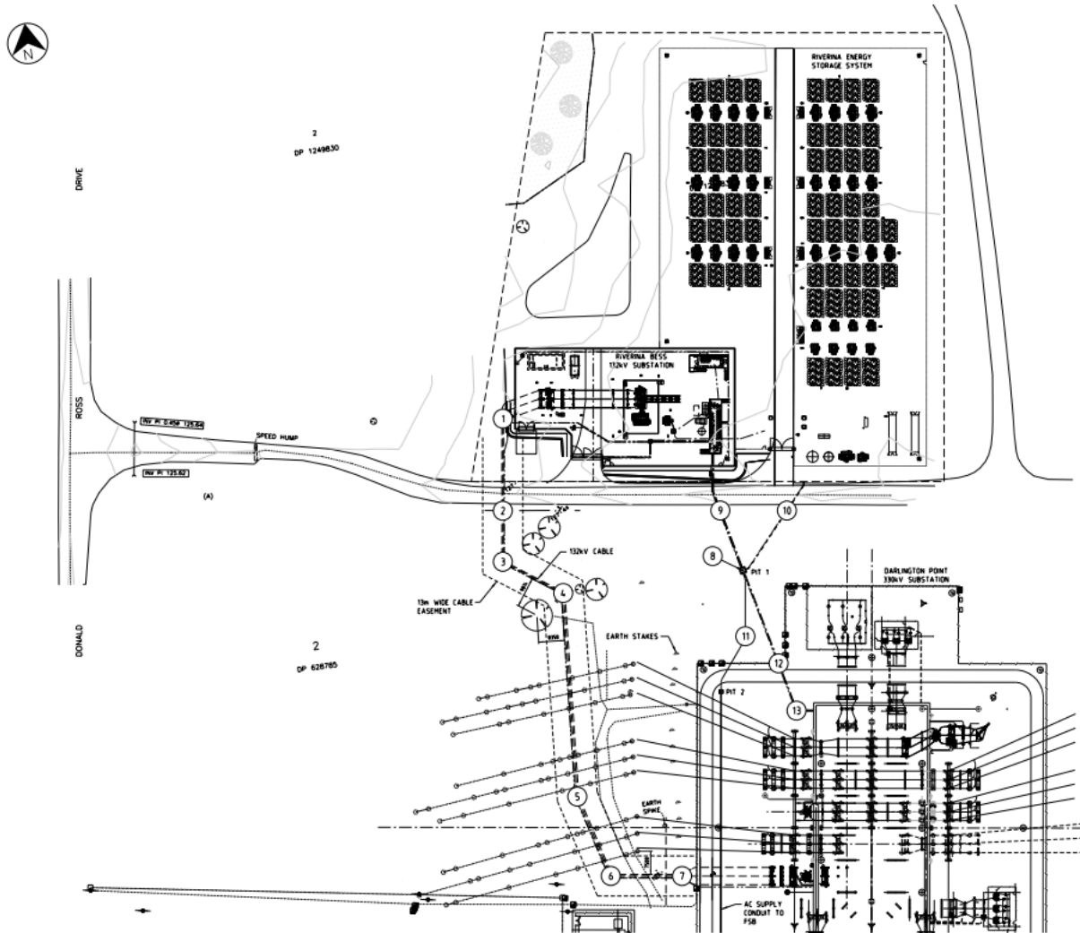
Figure 5 BESS and RBESS Sub construction layout on Lot 1 DP1249830 and Lot 2 DP1249830 and connection into the TG DP Sub via 132kV underground cable, control and communication conduits on Lot 2 DP628785
