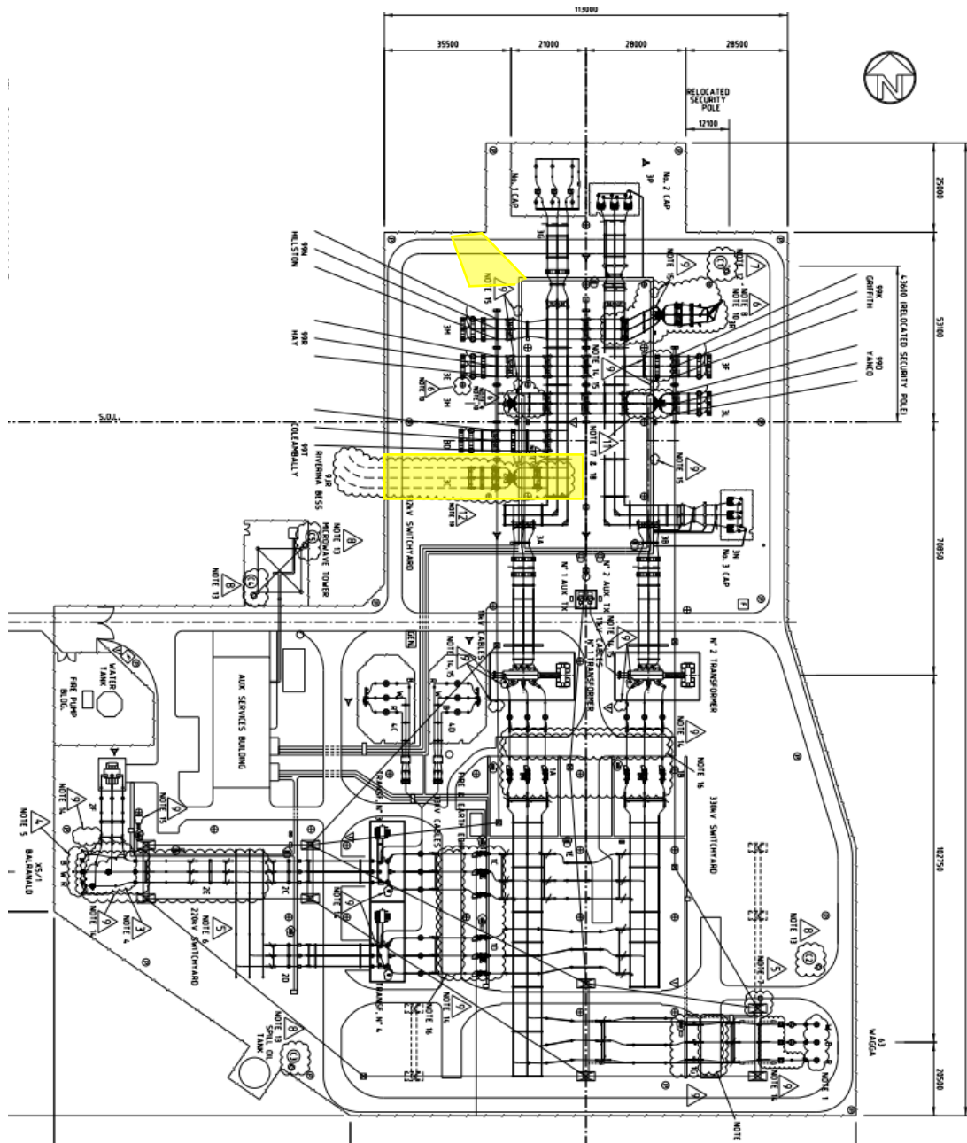
Figure 6 – 132kV Switch bay on Lot 2 DP628785 (Project works highlighted in YELLOW)
