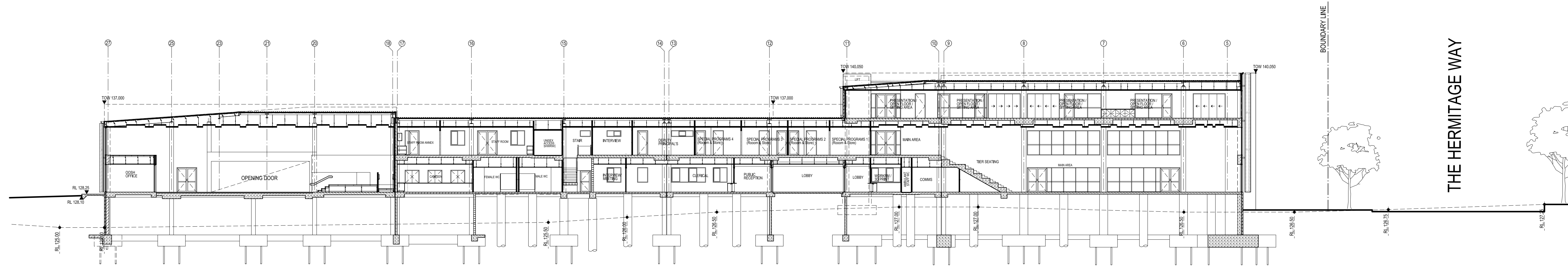
SECTION 01 SCALE 1:200
