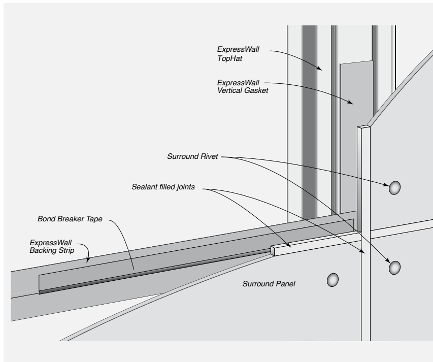
FIGURE 7.16 Joint Construction – Sealed Option
