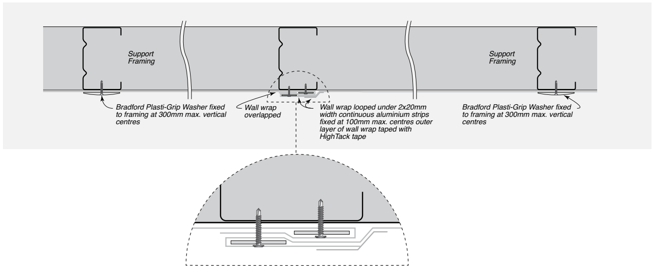
FIGURE 8.22 Vertical Wall Wrap Junction – Overlapped
