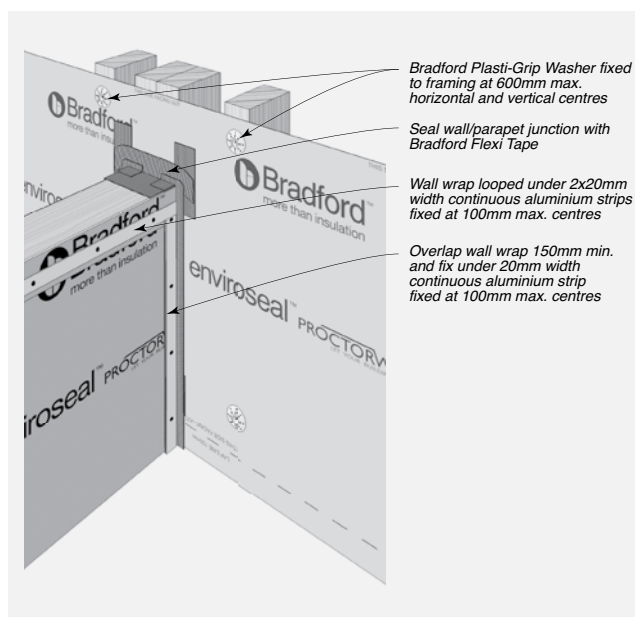
FIGURE 8.30 Wall Wrap Installation at Parapet Junction – Timber or Steel Framing
