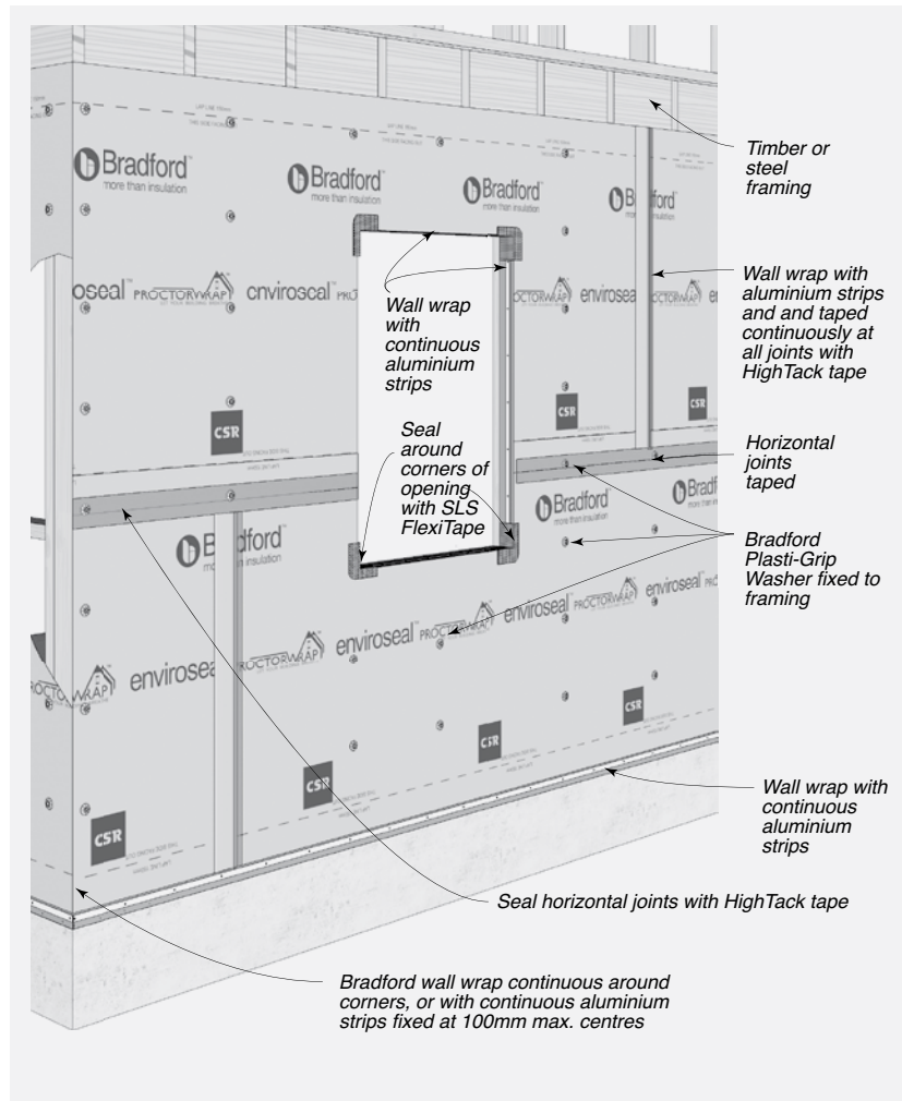
FIGURE 8.16 Typical Installation Overview Detail – Wall Wrap Soft Air Barrier
