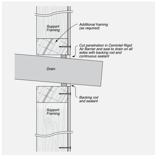
FIGURE 8.14 Junctions at Drain Penetration – Rigid Air Barrier – Timber or Steel Framing
