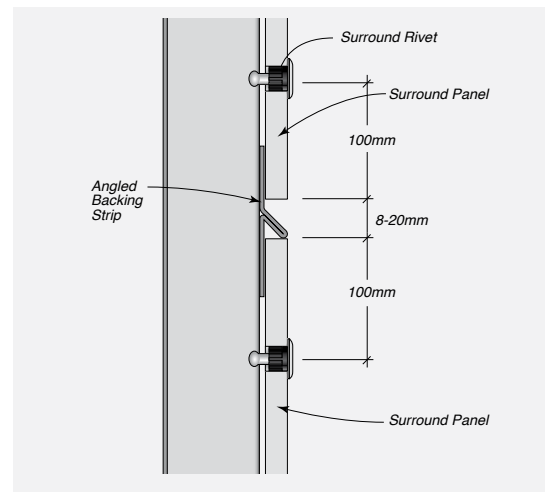
FIGURE 7.10 Horizontal Joint with Angled Backing Strip
