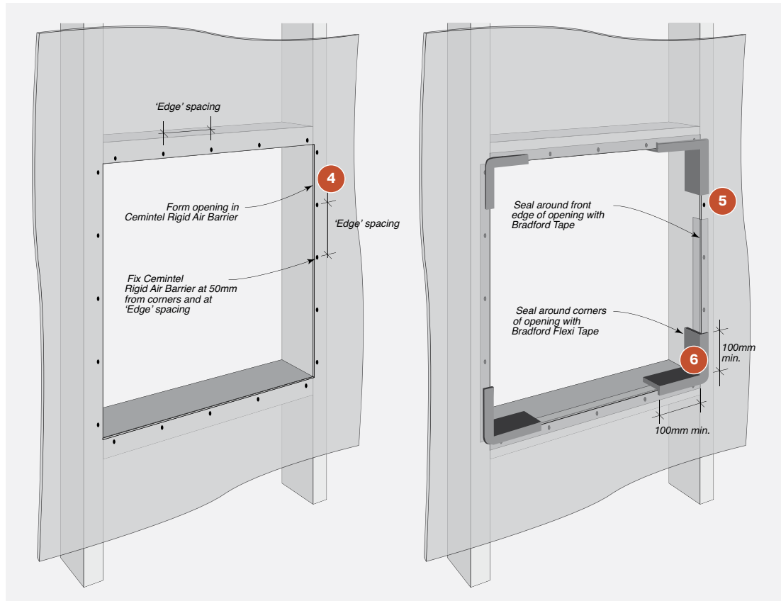
FIGURE 7.01 Treatment at Window/Door Openings – Rigid Air Barrier
