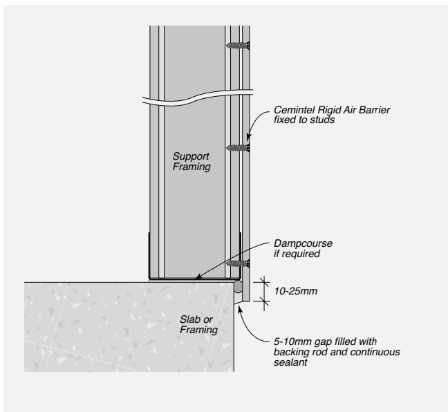
FIGURE 8.05 Junction at Base – Overhanging Framing – Rigid Air Barrier
