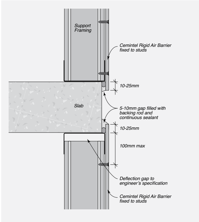
FIGURE 8.12 Control Joint Options – Horizontal
