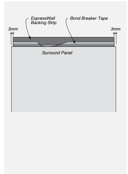
FIGURE 7.21 Backing Strip & Bond Breaker Tape
