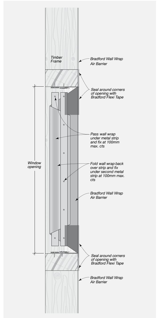
FIGURE 8.28 Wall Wrap Installation at Window/Door Opening
