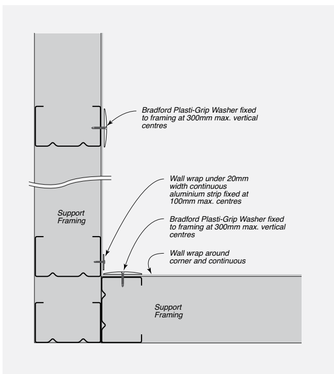
FIGURE 8.20 Internal Corner – Wall Wrap Continuous
