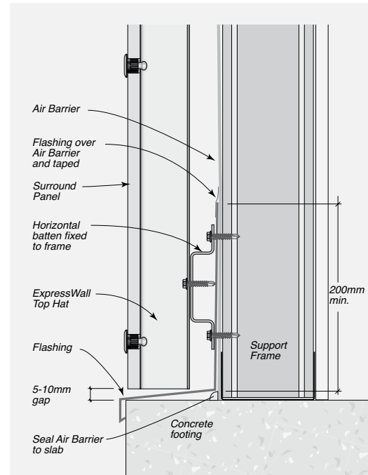
FIGURE 8.07 Base Detail – Drained
