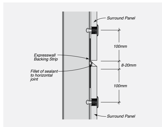
FIGURE 7.15 Horizontal Joint
