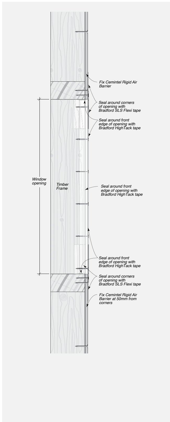
FIGURE 8.13 Treatment at Window/Door Openings – Rigid Air Barrier
