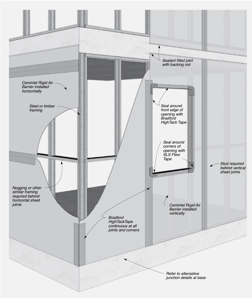
FIGURE 8.01 Typical Installation Overview – Rigid Air Barrier
