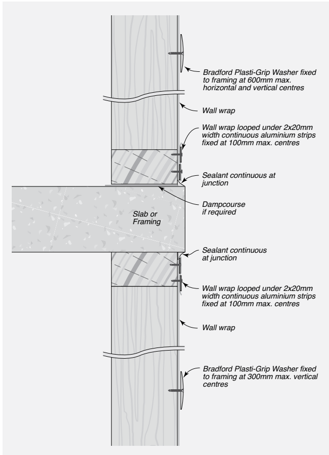
FIGURE 8.27 Wall Wrap Installation at Intermediate Level Junction – Timber Framing
