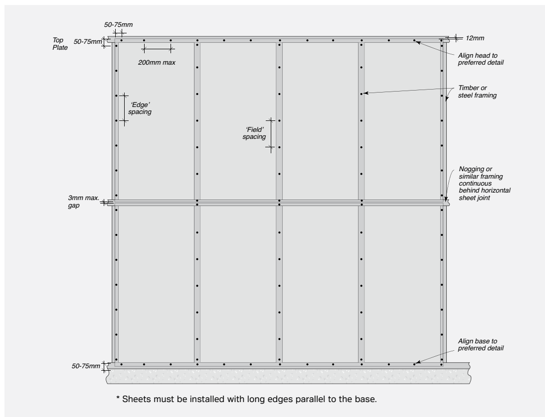
FIGURE 6.02 Sheet Fixing – Horizontal Sheeting* – Timber or Steel Framing
