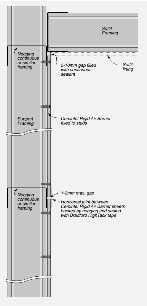
FIGURE 8.02 Junctions at Soffit, Base and Horizontal Sheet Joint – Rigid Air Barrier
