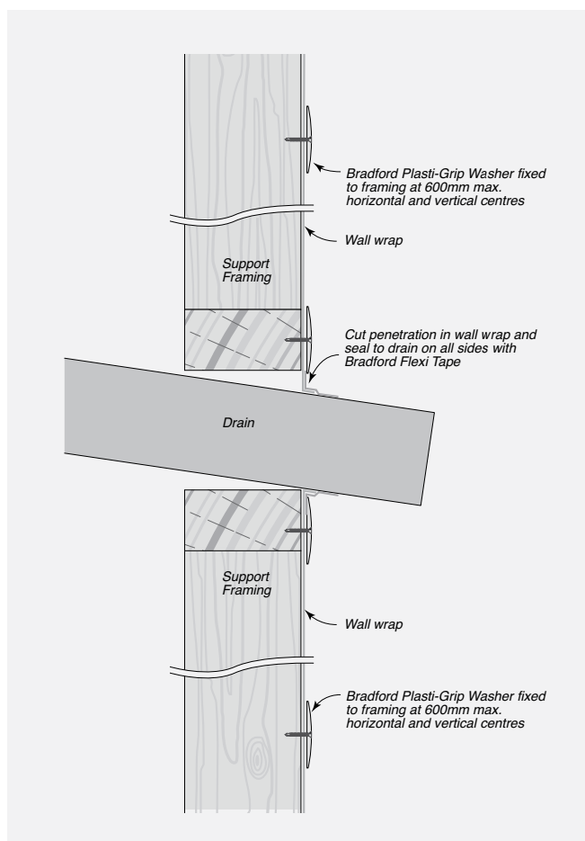
FIGURE 8.29 Wall Wrap Installation at Drain Penetration – Timber or Steel Framing
