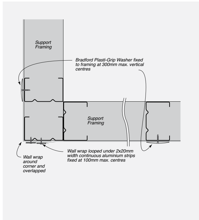
FIGURE 8.19 External Corner – Wall Wrap Overlapped
