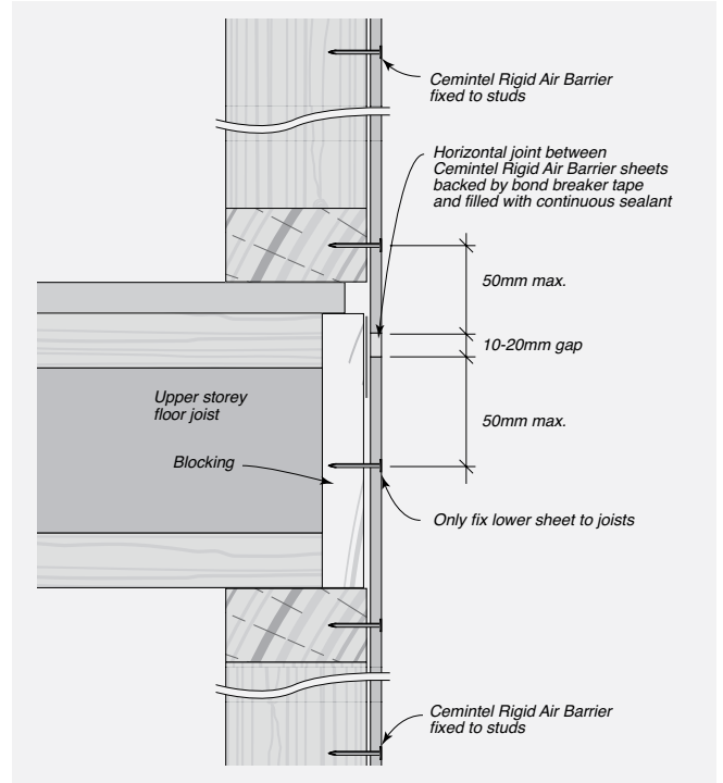
FIGURE 8.11 Junctions at Intermediate Level – Timber Framing – Rigid Air Barrier
