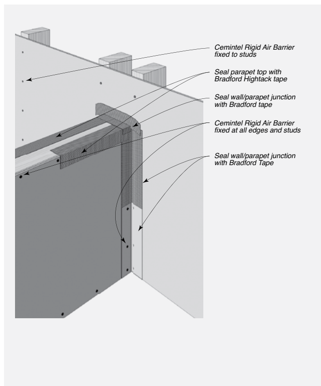
FIGURE 8.15 Installation at Parapet Junctions – Rigid Air Barrier – Timber or Steel Framing
