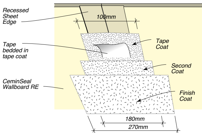
FIG 51: Flush-Set Jointing – Interior System Recessed Edge
