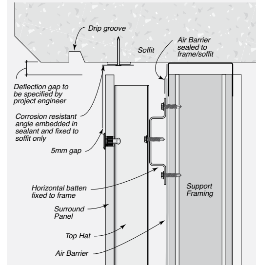
FIGURE 8.06 Eaves/Deflection Head – Ventilated
