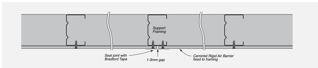
FIGURE 8.09 Vertical Junction – Rigid Air Barrier
