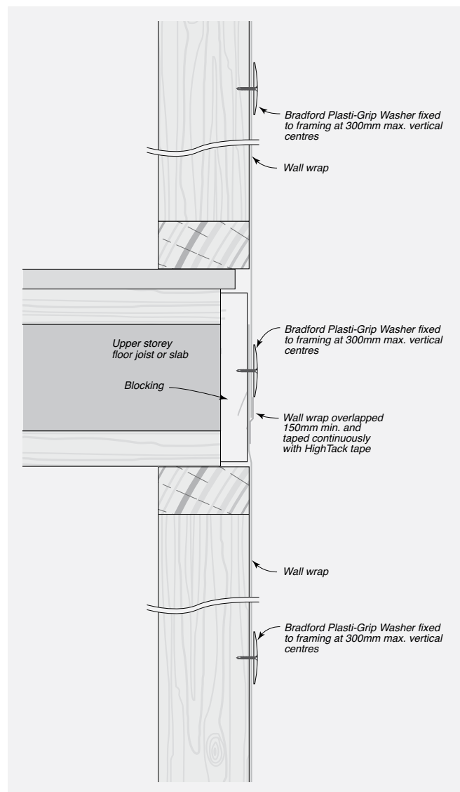
FIGURE 8.25 Wall Wrap Installation at inter storey Junction – Horizontal Overlapped and Taped Junction
