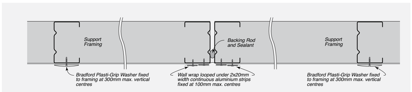
FIGURE 8.23 Vertical Wall Wrap Junction – At Control joint
