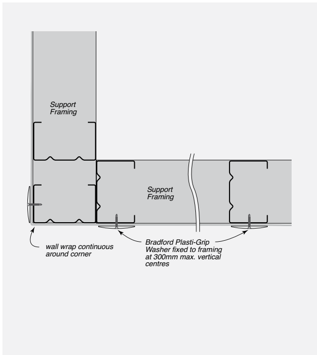
FIGURE 8.18 External Corner – Wall Wrap Continuous
