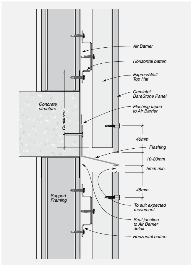
FIGURE 8.12 Control Joint Options – Horizontal
