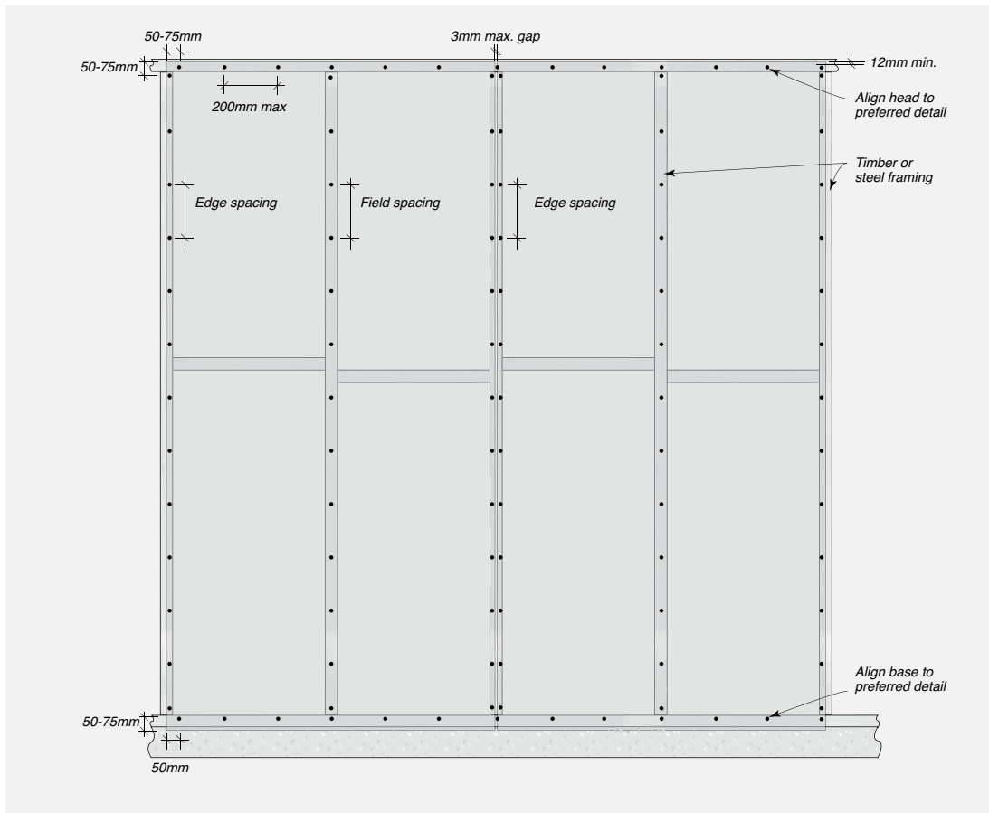
FIGURE 6.01 Sheet Fixing – Vertical Sheeting – Timber or Steel Framing
