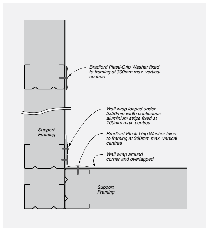
FIGURE 8.21 Internal Corner – Wall Wrap Overlapped
