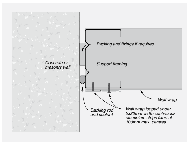
FIGURE 8.24 Wall Wrap Abutment to Concrete or Masonry Wall
