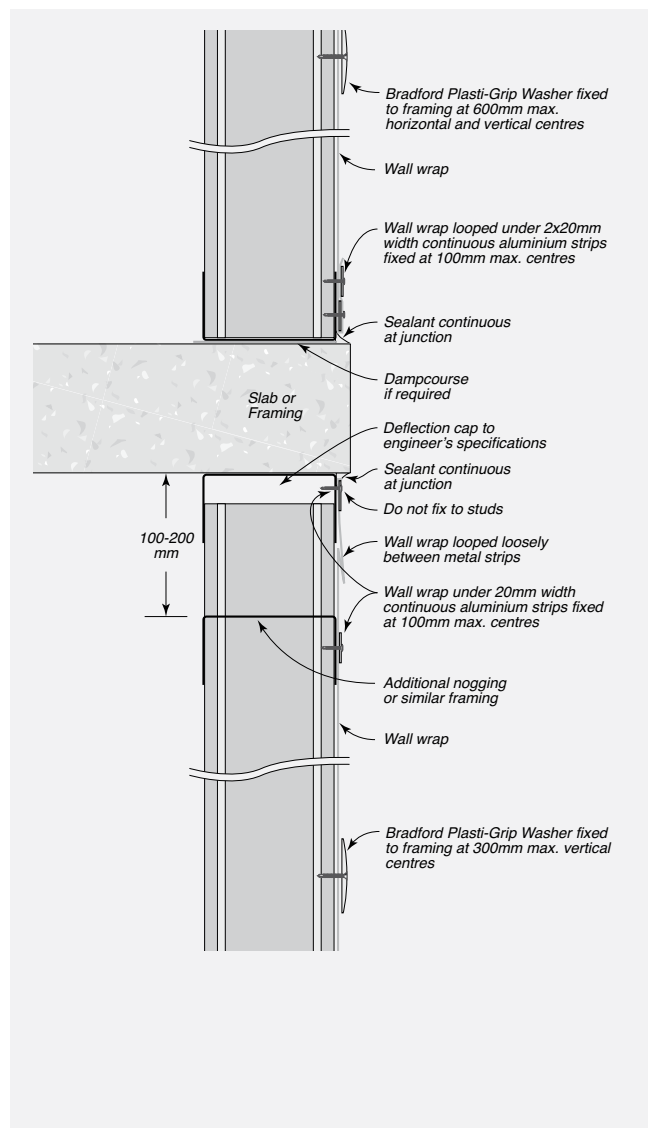
FIGURE 8.26 Wall Wrap Installation at Intermediate Level Junction – Steel Framing with Deflection Head
