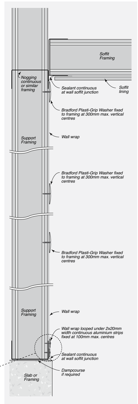
FIGURE 8.17 Wall Wrap Installation to Wall, Soffit and Base
