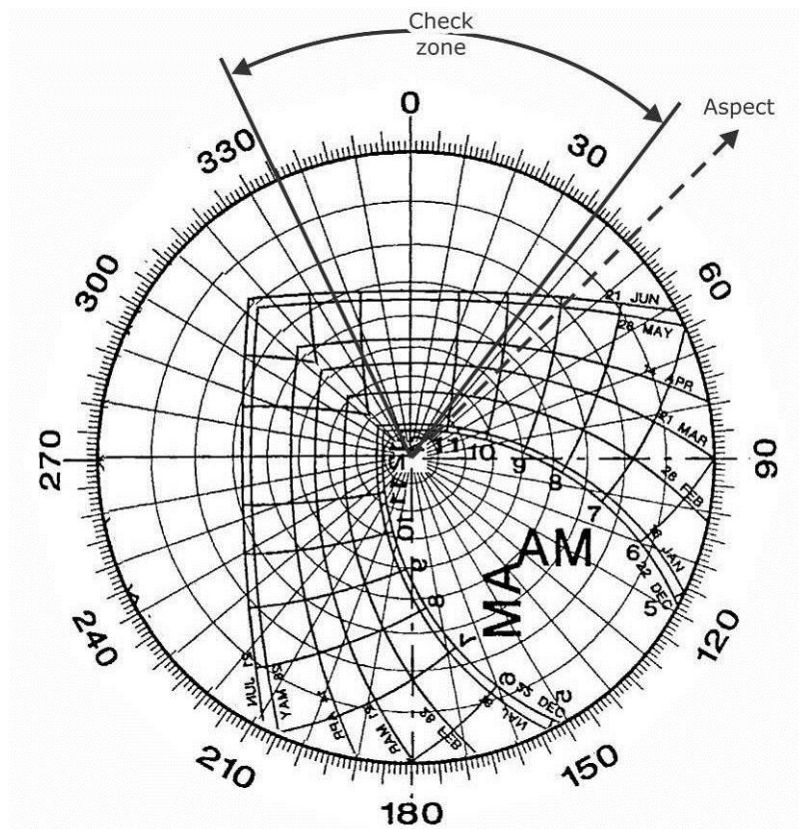
Figure B6: Sun Chart for Aspect 045°
