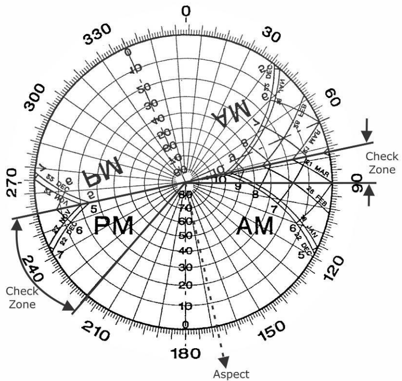
Figure B20: Sun Chart for Aspect 168°
