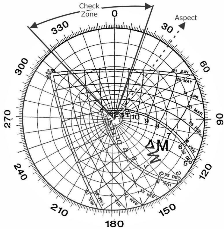
Figure B5: Sun Chart for Aspect 036°
