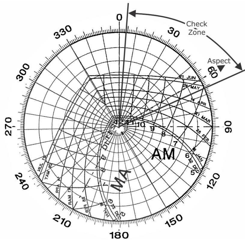
Figure B9: Sun Chart for Aspect 060°
