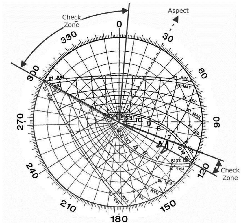
Figure B4: Sun Chart for Aspect 029°
