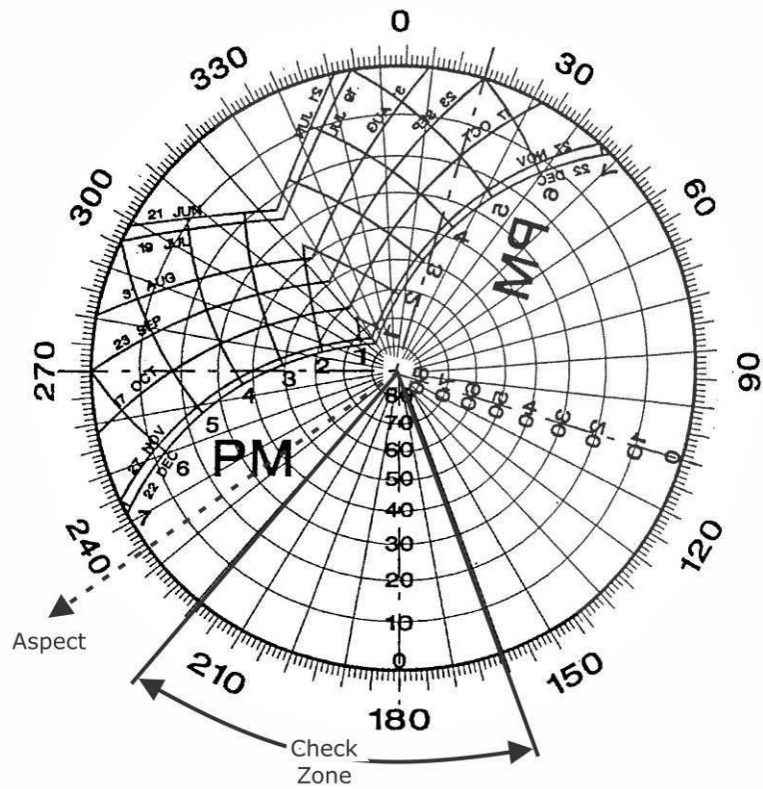
Figure B23: Sun Chart for Aspect 234°
