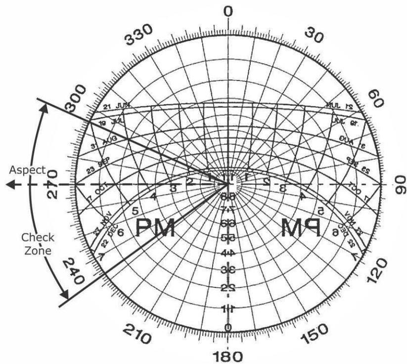
Figure B28: Sun Chart for Aspect 270°
