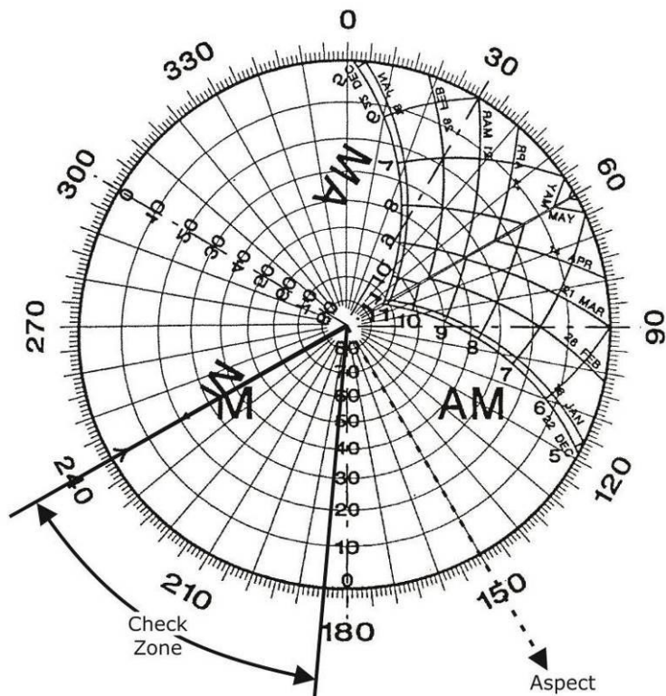
Figure B18: Sun Chart for Aspect 150°
