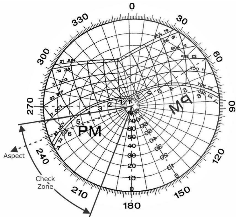
Figure B27: Sun Chart for Aspect 254°
