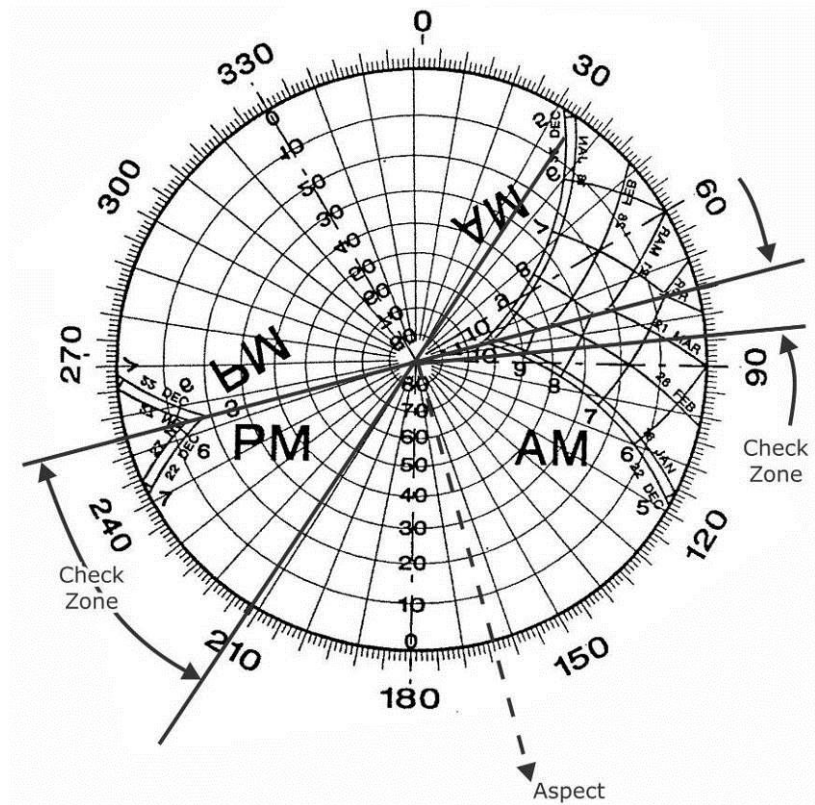
Figure B19: Sun Chart for Aspect 164°
