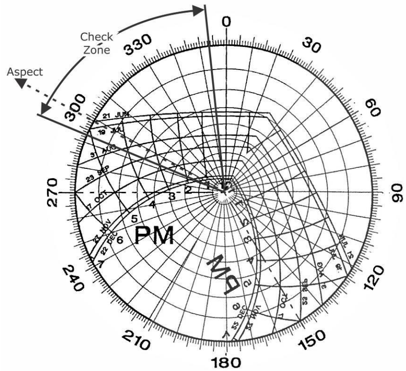
Figure B29: Sun Chart for Aspect 299°
