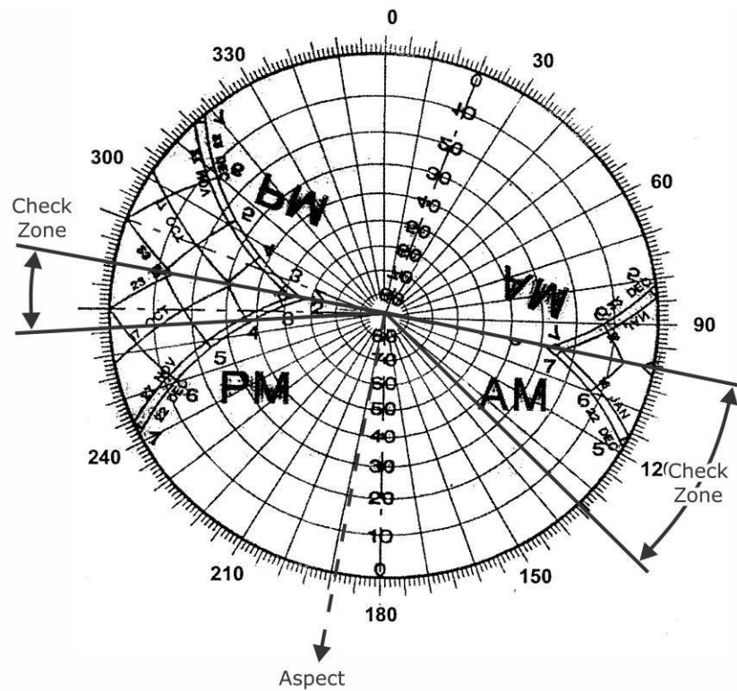
Figure B21: Sun Chart for Aspect 189°
