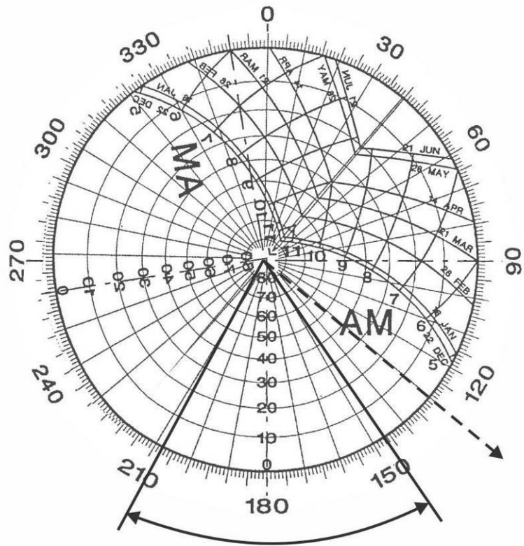
Figure B17: Sun Chart for Aspect 130°
