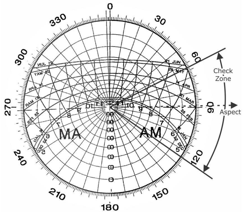
Figure B13: Sun Chart for Aspect 089°
