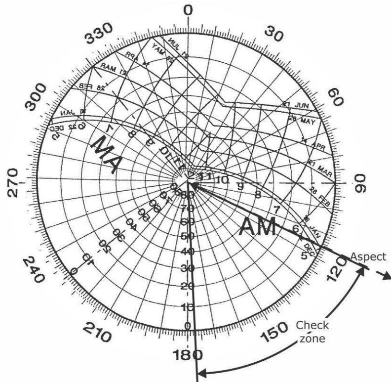
Figure B15: Sun Chart for Aspect 115°
