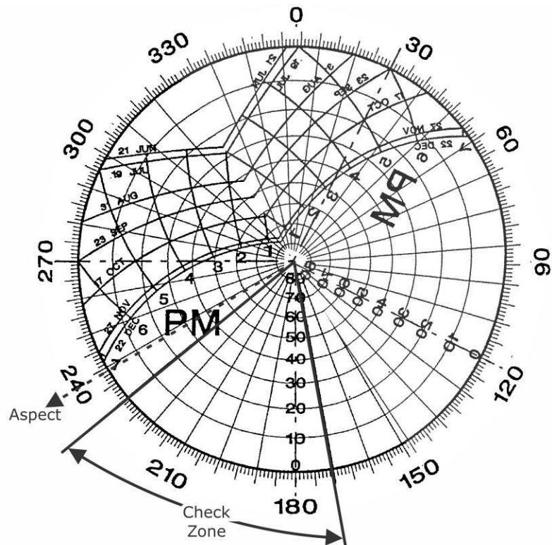
Figure B24: Sun Chart for Aspect 239°
