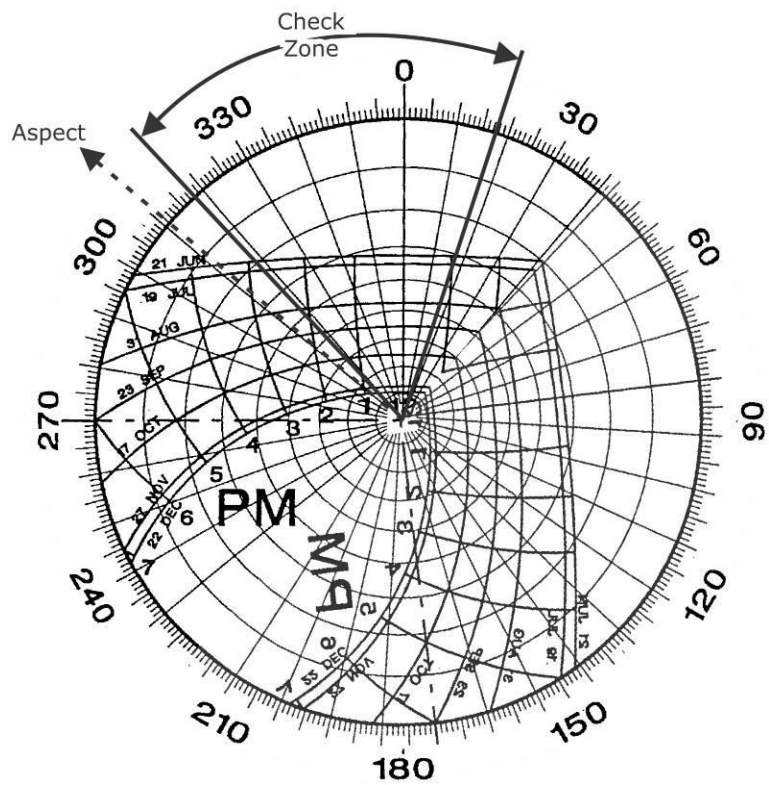
Figure B30: Sun Chart for Aspect 311°
