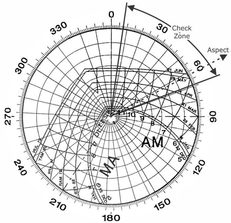
Figure B10: Sun Chart for Aspect 062°
