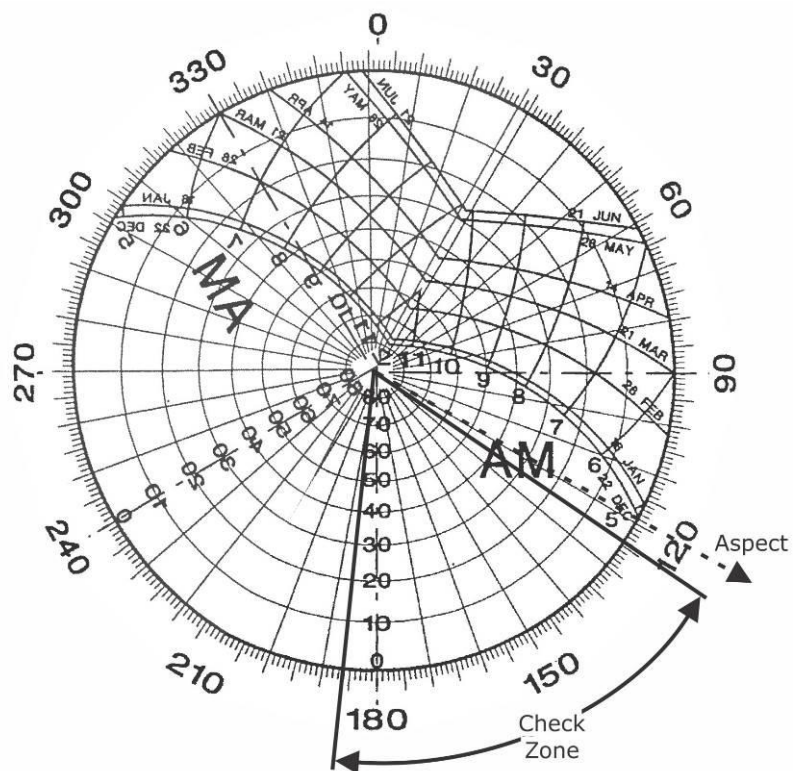
Figure B16: Sun Chart for Aspect 119°
