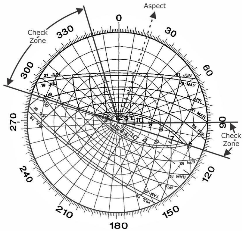
Figure B3: Sun Chart for Aspect 018°
