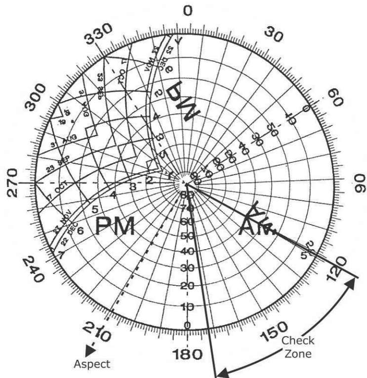
Figure B22: Sun Chart for Aspect 209°
