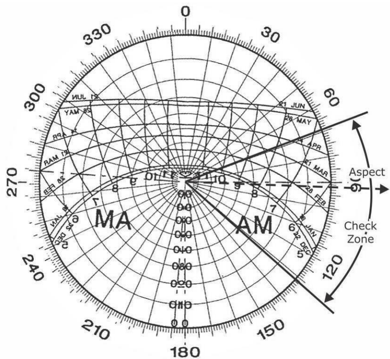
Figure B14: Sun Chart for Aspect 092°
