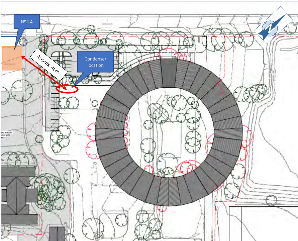
Figure 6: Proposed location of mechanical plant
