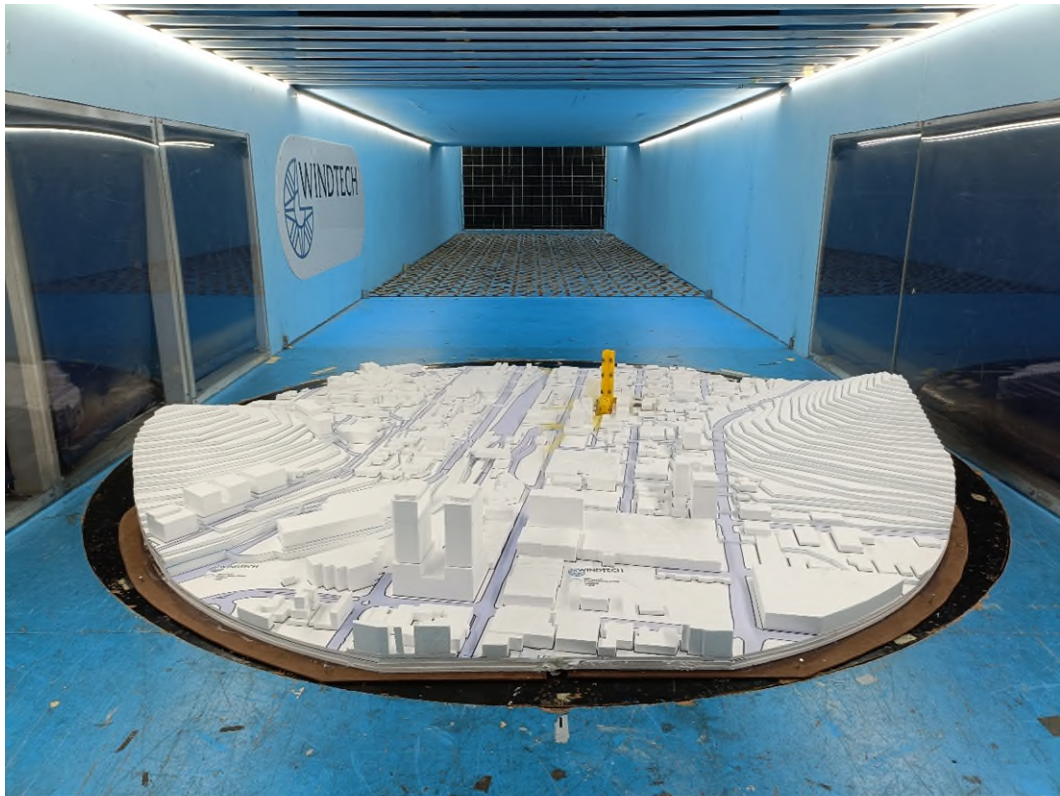
Figure 1d: Photograph of the Wind Tunnel Model (view from the south)
