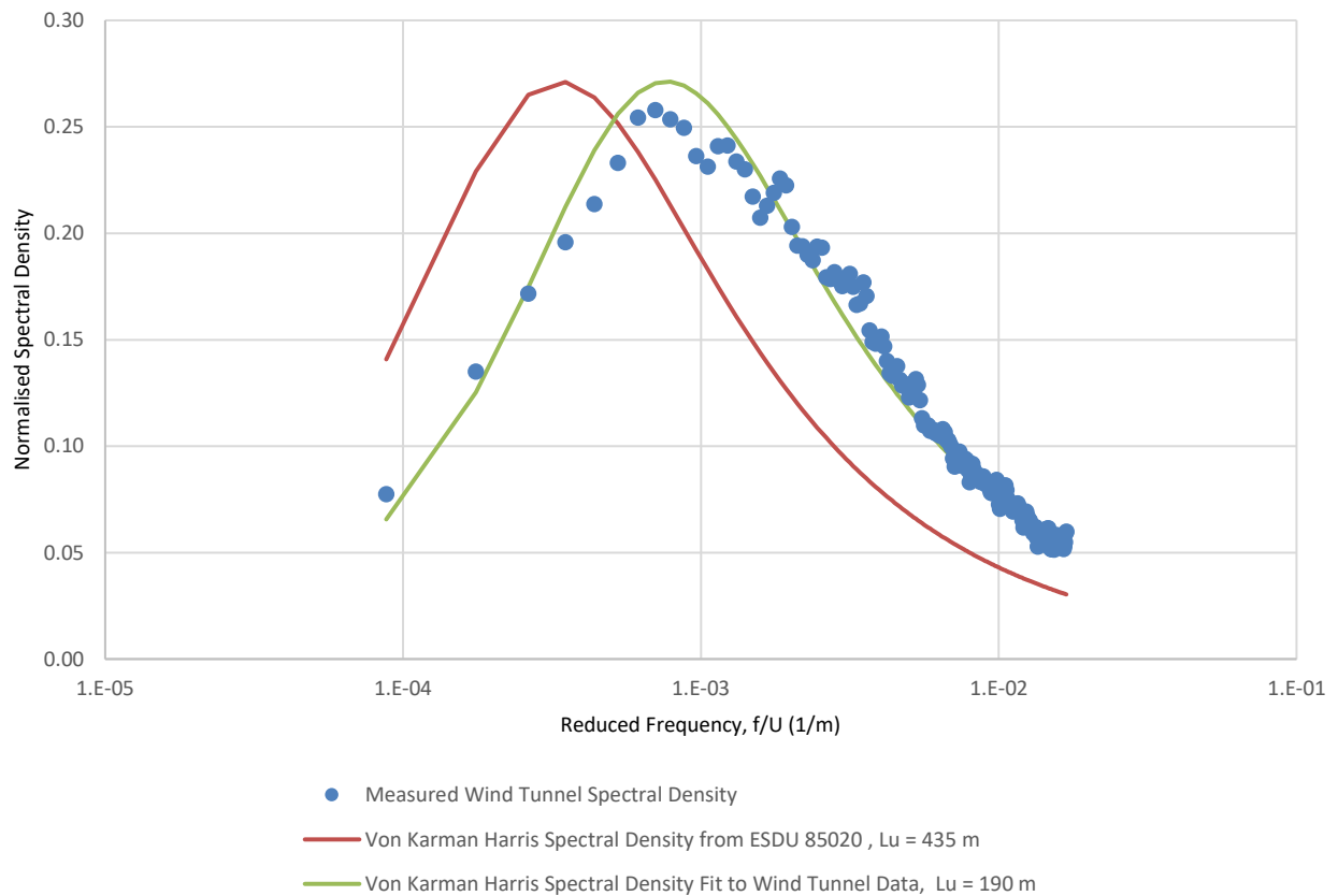
Longitudinal Spectra Density for Open Terrain ( 0.02\text{m} < z_0 < 0.03\text{m} ) (TC2) at a 1:400 Scale
