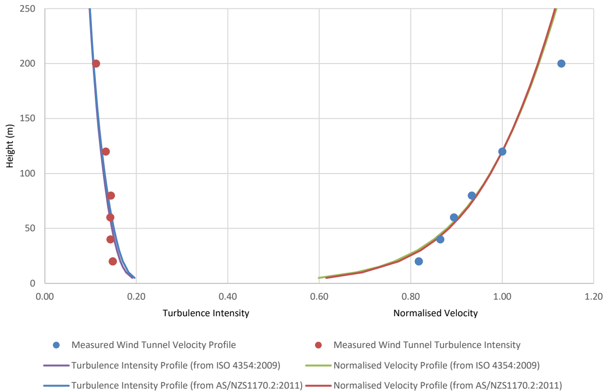
Mean Velocity and Turbulence Intensity for Open Terrain ( 0.02\text{m} < z_0 < 0.03\text{m} ) (TC2) at a 1:400 Scale
