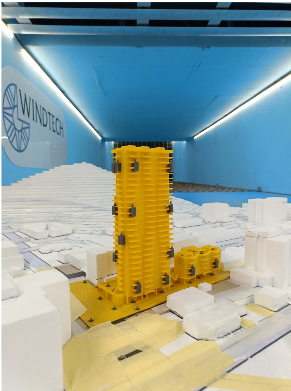
Figure 1a: Photograph of the Wind Tunnel Model (view from the north-west)
