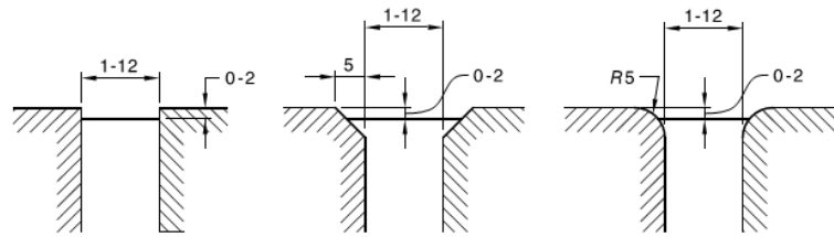
(a) Continuous paving units — Level surface
