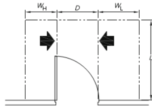
(e) Hinge-side approach, door opens towards user
