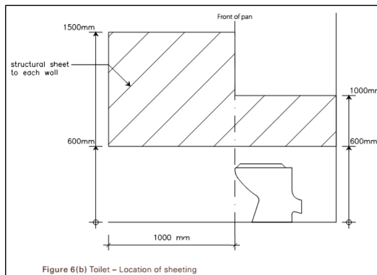
Figure 6(b) Toilet - Location of sheeting
