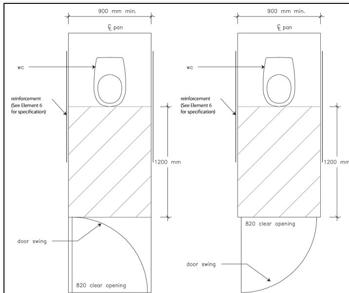
Figure 3(a) Silver level ground (or entry) level toilet layout and space requirements in a separate room.
