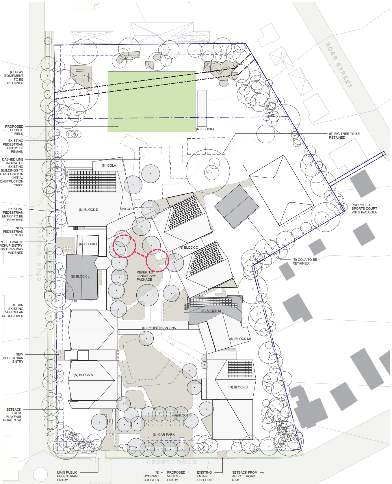
2 PROPOSED SITE PLAN 1:500
