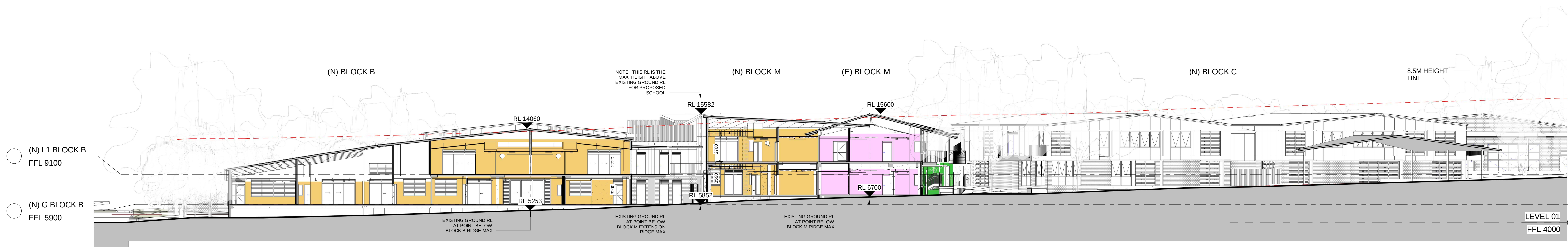
4 (N) SECTION 4 1:200
