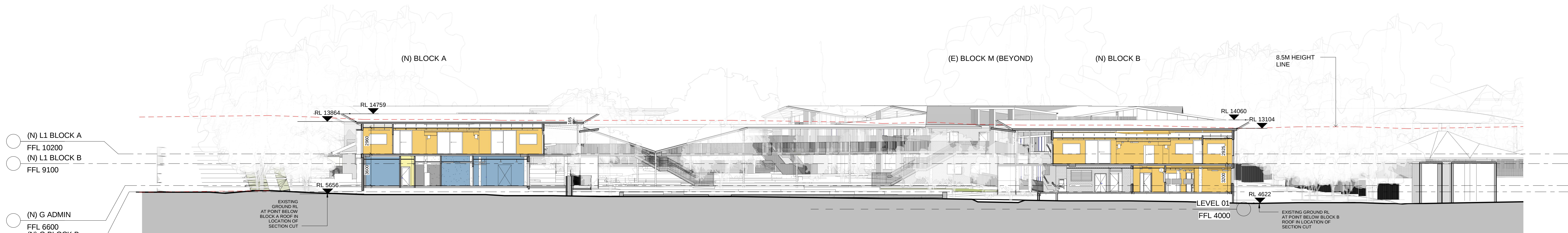
1 (N) SECTION 1 1:200
