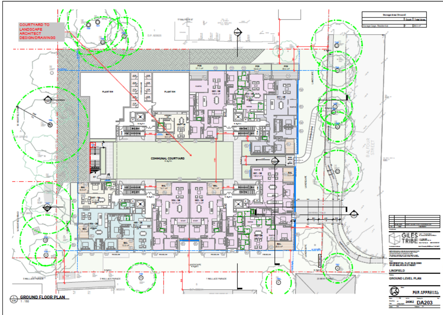
Figure 2 – Ground floor site plan for proposed apartment building at 19 – 25 Balfour Street, Lindfield (for detail see Giles Tribe Architects 2025), note building footprint does not encroach on the TPZ of any significant trees (from A Scales 2025)
