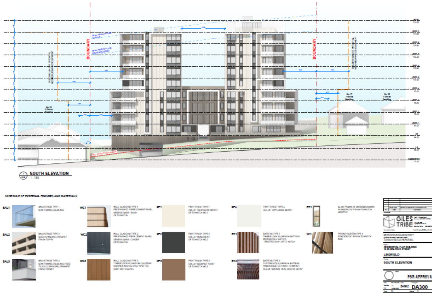
Figure 3 – Image of South Elevation of proposed apartment building at 19 – 25 Balfour Street, Lindfield (for detail see Giles Tribe Architects 2025)
