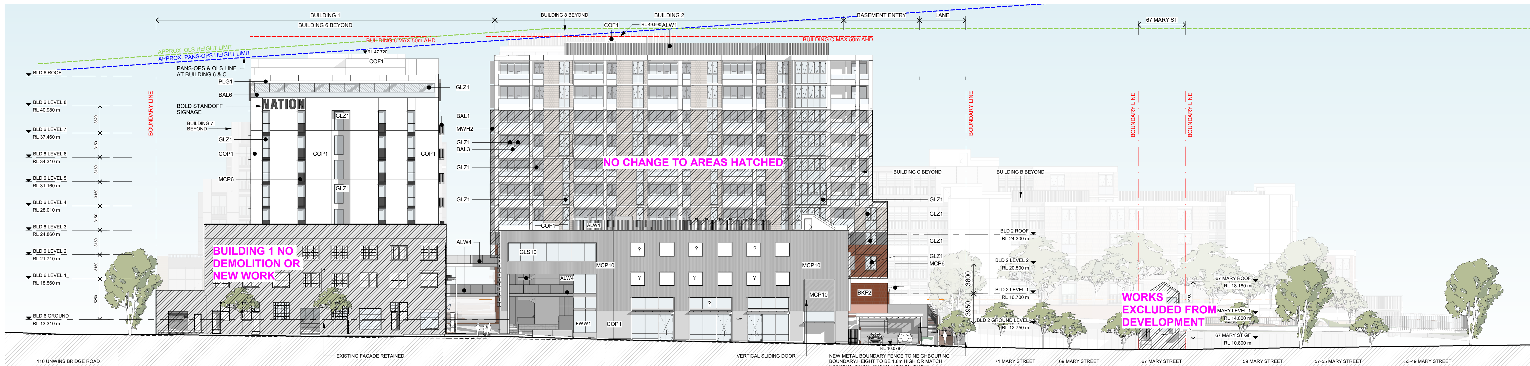
1 SOUTH-WEST - MARY ST SCALE 1 : 250
