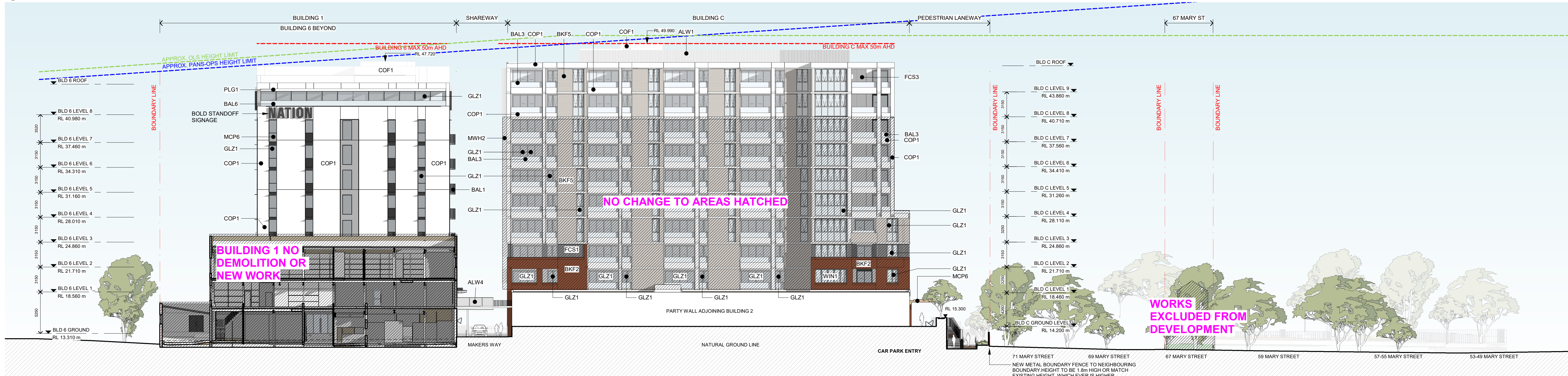
2 SOUTH-WEST - BUILDING C, 1 SCALE 1 : 250
