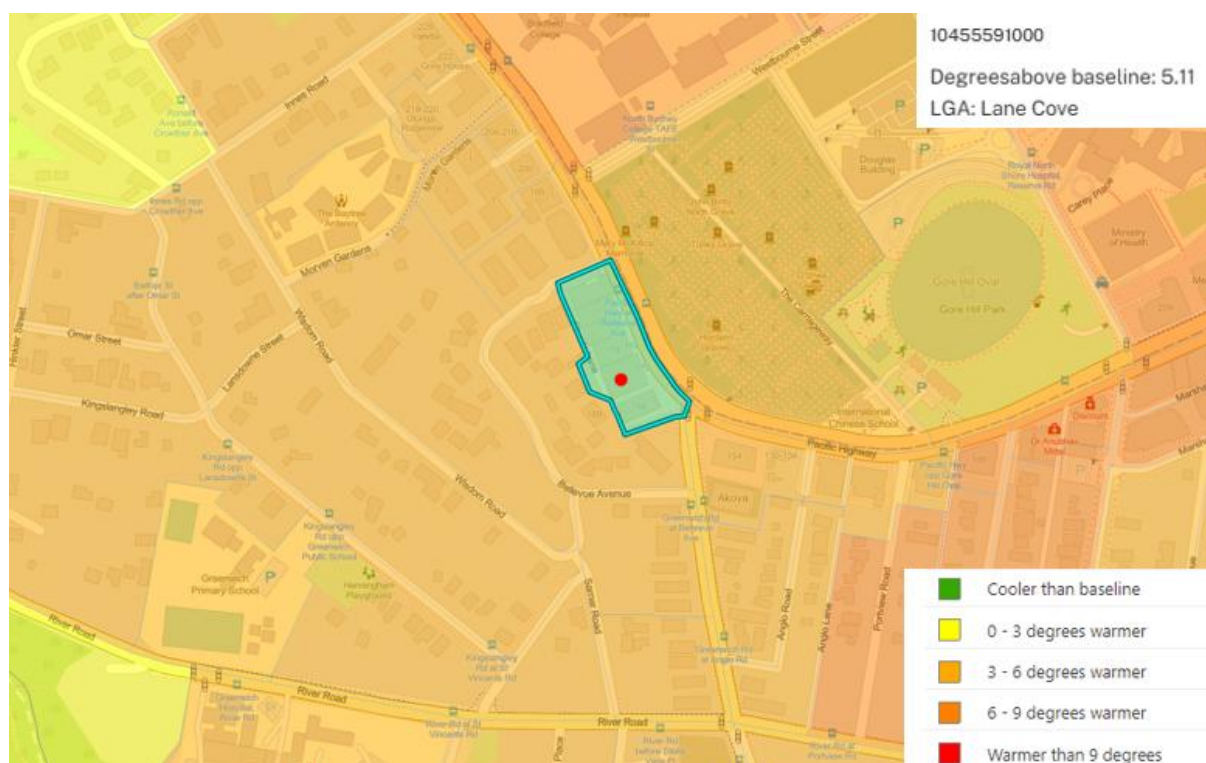
Figure 3: Urban Heat Island Effect at the site (Source: SEED Database, 2016)
