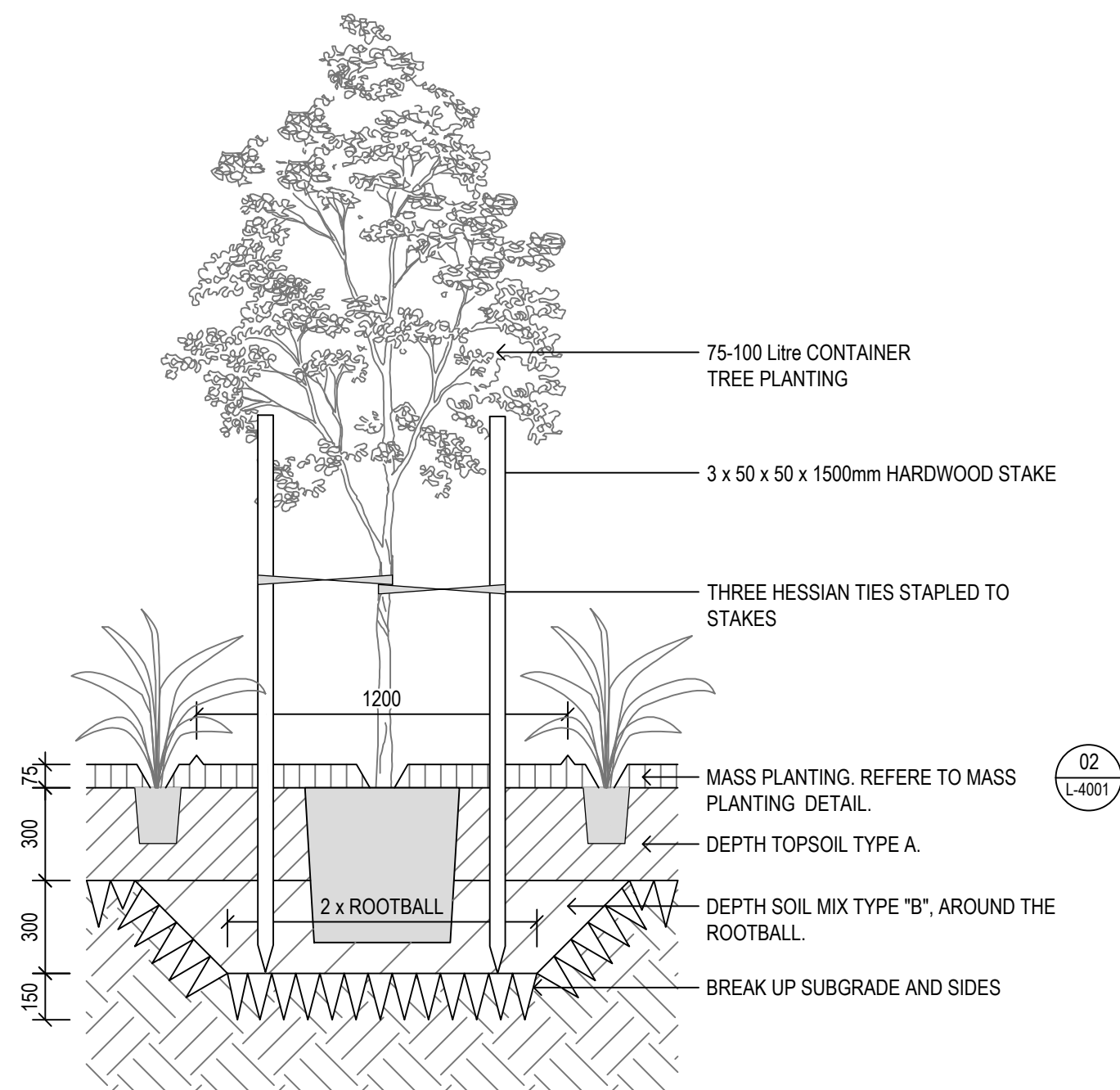
05 TREE PLANTING IN MASS PLANTING TYPICAL SECTION 1:20@ B1
