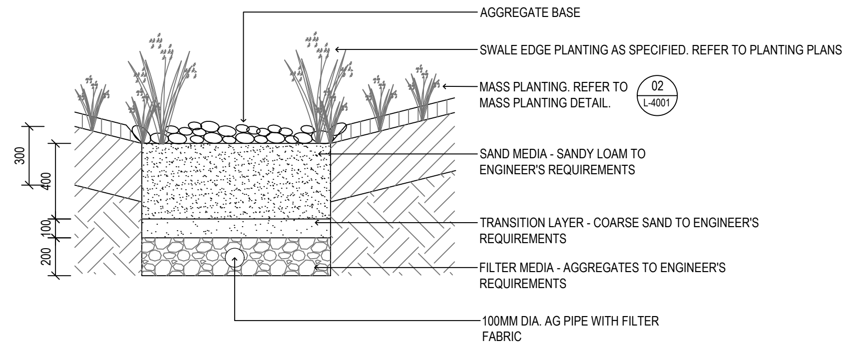
03 PLANTING TO BIO-RETENTION SWALE TYPICAL SECTION 1:20@ B1
