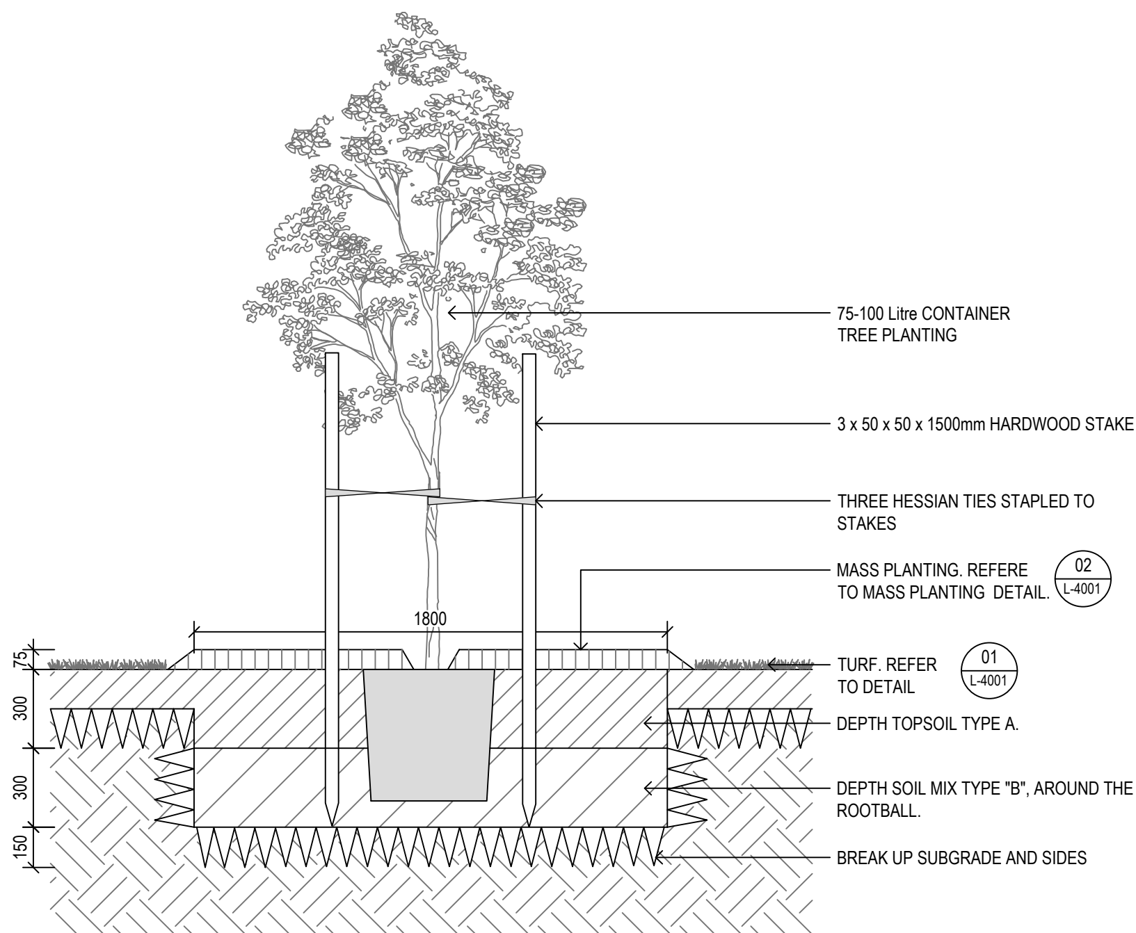
04 TREE PLANTING IN TURF TYPICAL SECTION 1:20@ B1
