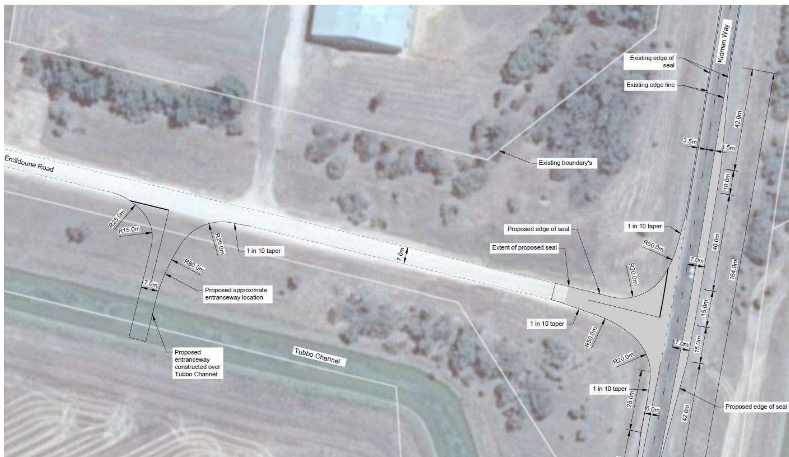
Figure 3-17 Access concept design
