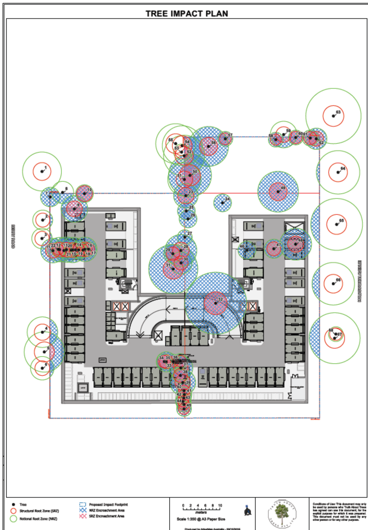
Figure 8- Tree impact plan showing a basement level.
