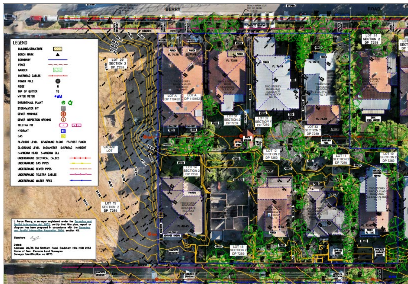
Figure 1 – Provided survey plan.
