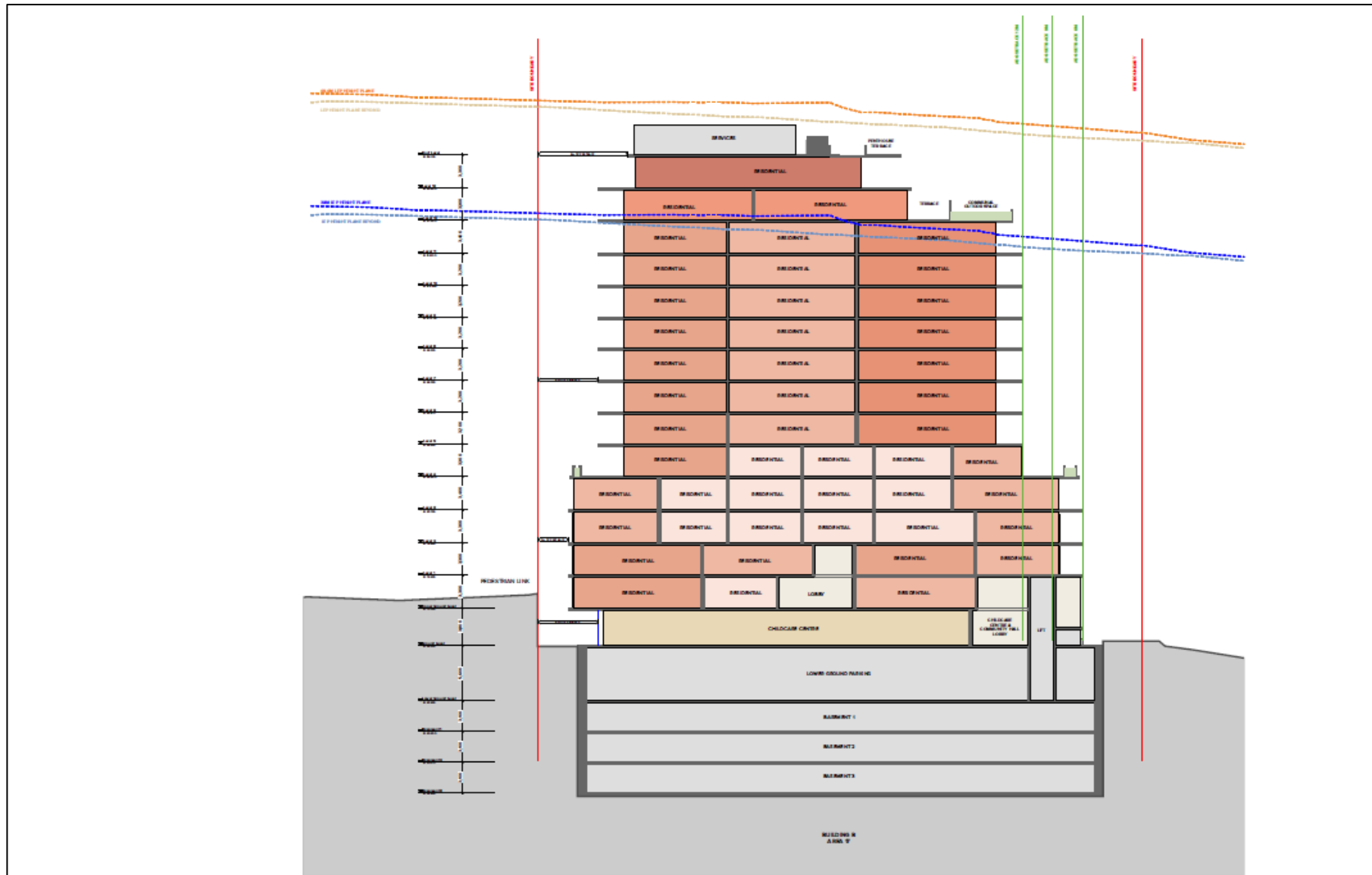
Figure 4- Section CC Plan.
